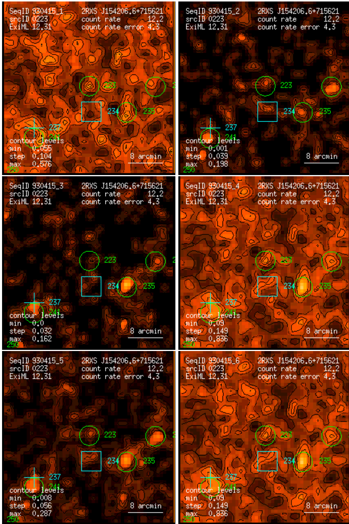
Figure 223: RASS 930415: detection 0223: band rate images, Gaussian filter: (1) PSPC channels 11 – 41, (2) 52 – 90, (3) 91 – 201, (4) 11 – 235, (5) 52 – 201, (6) 11 – 201. Broad band rates in counts/ks. Band rate contour levels in counts/ks/arcmin 2 .
