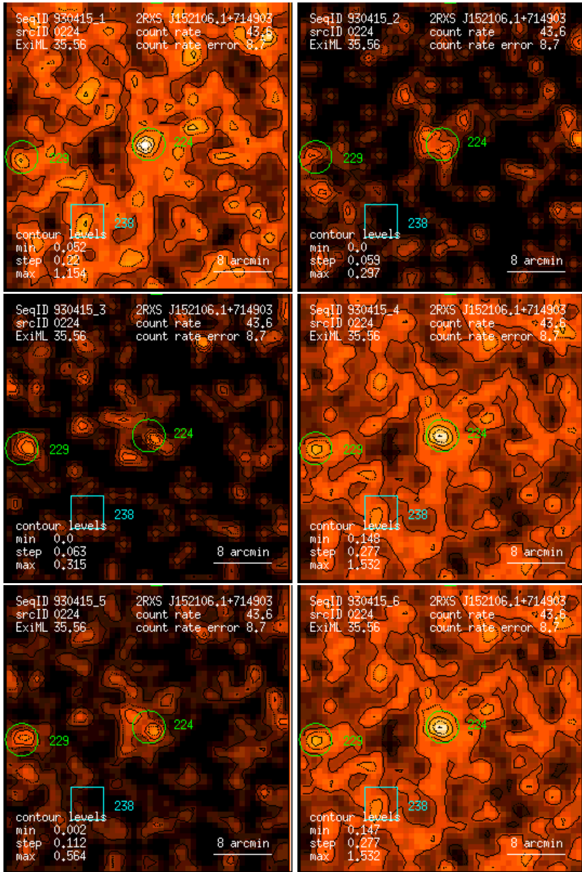
Figure 224: RASS 930415: detection 0224: band rate images, Gaussian filter: (1) PSPC channels 11 – 41, (2) 52 – 90, (3) 91 – 201, (4) 11 – 235, (5) 52 – 201, (6) 11 – 201. Broad band rates in counts/ks. Band rate contour levels in counts/ks/arcmin 2 .
