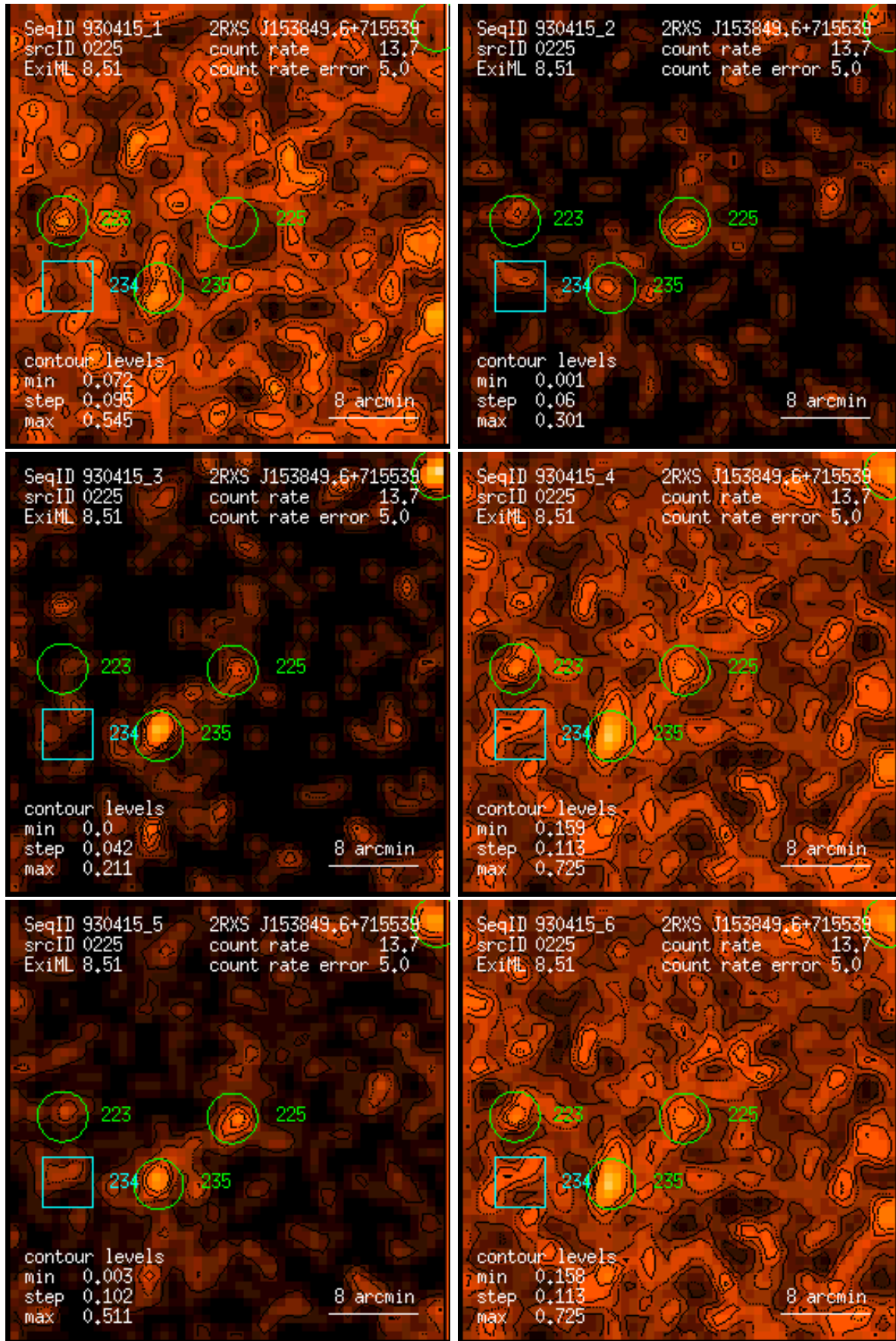
Figure 225: RASS 930415: detection 0225: band rate images, Gaussian filter: (1) PSPC channels 11 – 41, (2) 52 – 90, (3) 91 – 201, (4) 11 – 235, (5) 52 – 201, (6) 11 – 201. Broad band rates in counts/ks. Band rate contour levels in counts/ks/arcmin 2 .
