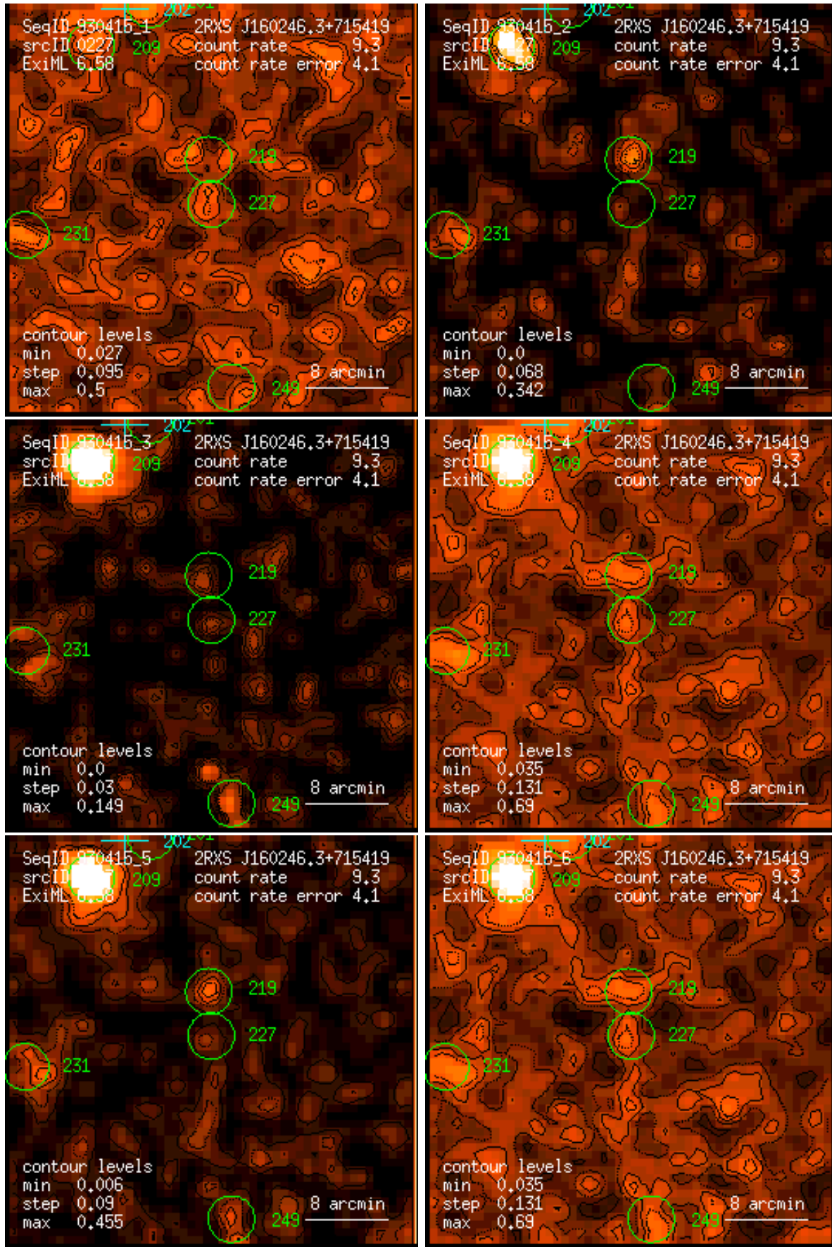
Figure 227: RASS 930415: detection 0227: band rate images, Gaussian filter: (1) PSPC channels 11 – 41, (2) 52 – 90, (3) 91 – 201, (4) 11 – 235, (5) 52 – 201, (6) 11 – 201. Broad band rates in counts/ks. Band rate contour levels in counts/ks/arcmin 2 .
