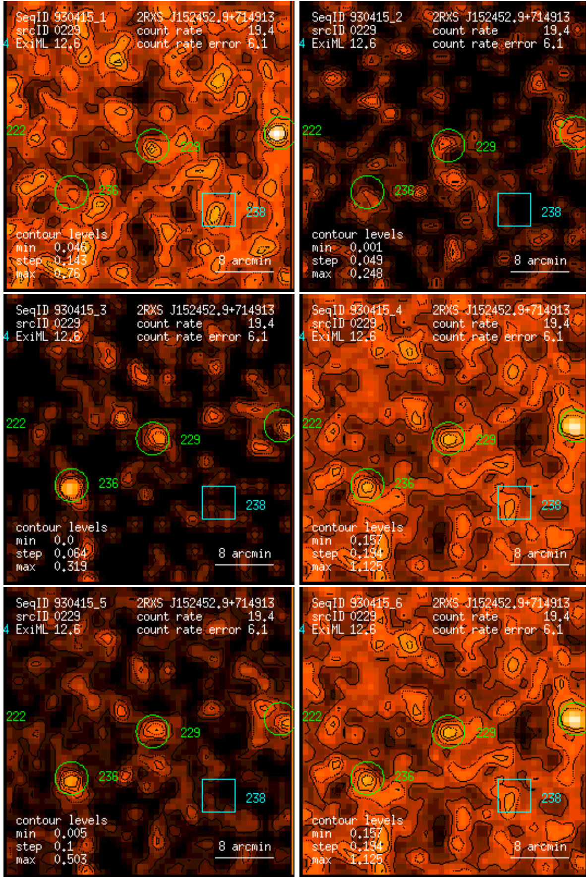
Figure 229: RASS 930415: detection 0229: band rate images, Gaussian filter: (1) PSPC channels 11 – 41, (2) 52 – 90, (3) 91 – 201, (4) 11 – 235, (5) 52 – 201, (6) 11 – 201. Broad band rates in counts/ks. Band rate contour levels in counts/ks/arcmin 2 .
