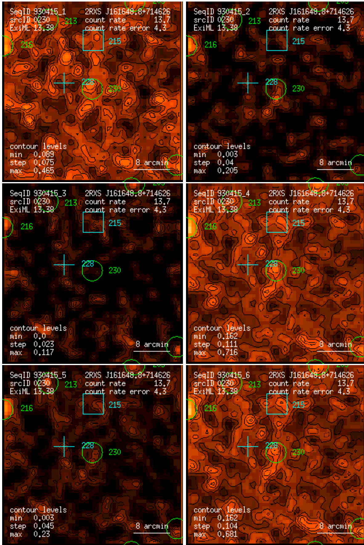
Figure 230: RASS 930415: detection 0230: band rate images, Gaussian filter: (1) PSPC channels 11 – 41, (2) 52 – 90, (3) 91 – 201, (4) 11 – 235, (5) 52 – 201, (6) 11 – 201. Broad band rates in counts/ks. Band rate contour levels in counts/ks/arcmin 2 .
