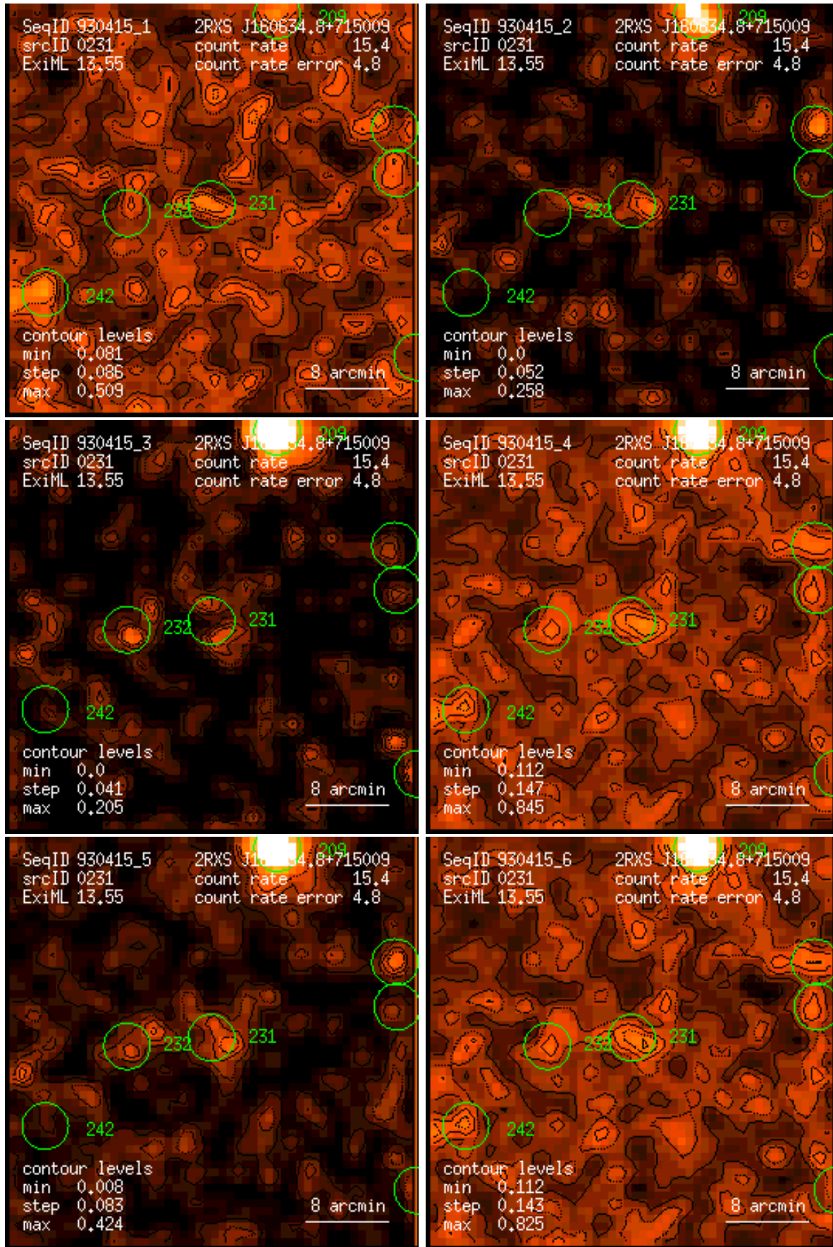
Figure 231: RASS 930415: detection 0231: band rate images, Gaussian filter: (1) PSPC channels 11 – 41, (2) 52 – 90, (3) 91 – 201, (4) 11 – 235, (5) 52 – 201, (6) 11 – 201. Broad band rates in counts/ks. Band rate contour levels in counts/ks/arcmin 2 .
