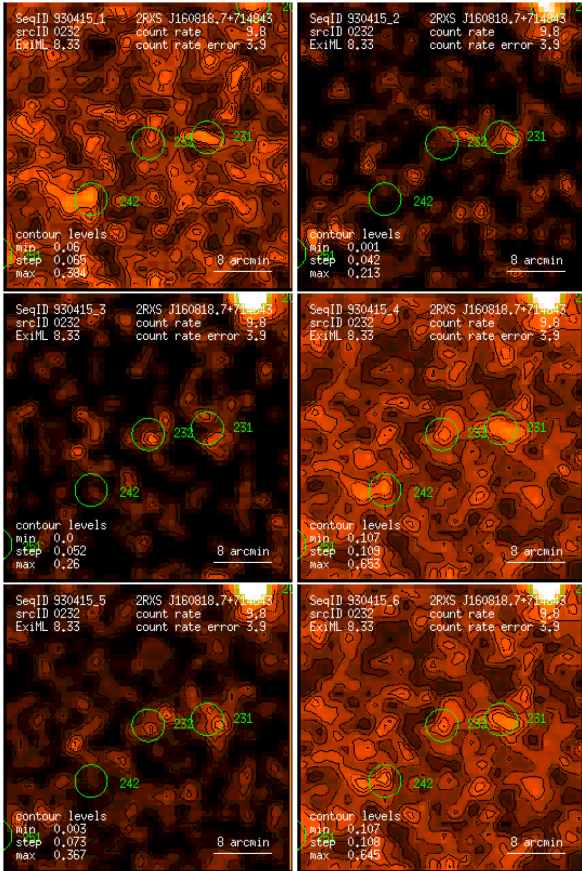
Figure 232: RASS 930415: detection 0232: band rate images, Gaussian filter: (1) PSPC channels 11 – 41, (2) 52 – 90, (3) 91 – 201, (4) 11 – 235, (5) 52 – 201, (6) 11 – 201. Broad band rates in counts/ks. Band rate contour levels in counts/ks/arcmin 2 .
