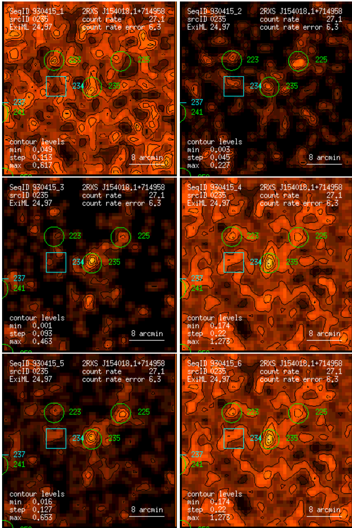
Figure 235: RASS 930415: detection 0235: band rate images, Gaussian filter: (1) PSPC channels 11 – 41, (2) 52 – 90, (3) 91 – 201, (4) 11 – 235, (5) 52 – 201, (6) 11 – 201. Broad band rates in counts/ks. Band rate contour levels in counts/ks/arcmin 2 .
