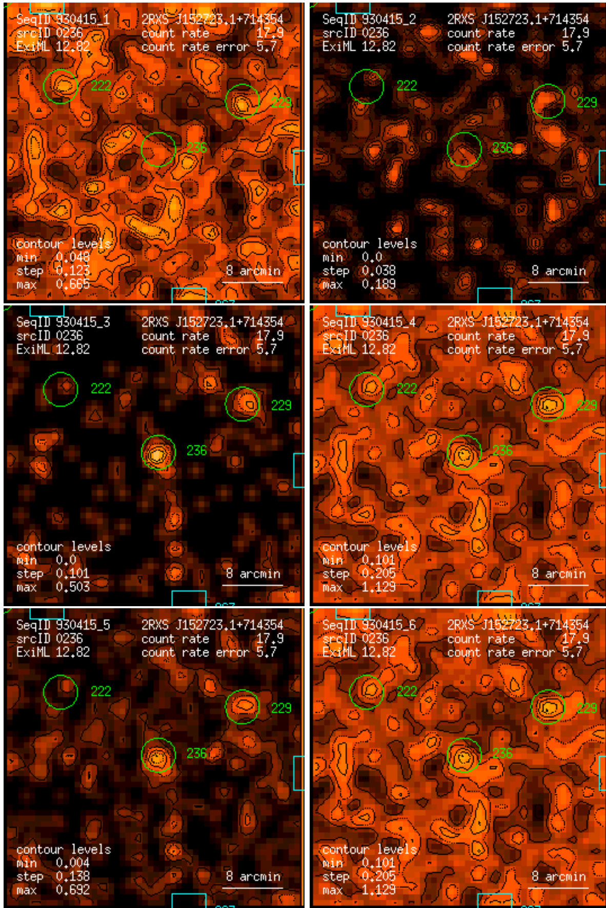
Figure 236: RASS 930415: detection 0236: band rate images, Gaussian filter: (1) PSPC channels 11 – 41, (2) 52 – 90, (3) 91 – 201, (4) 11 – 235, (5) 52 – 201, (6) 11 – 201. Broad band rates in counts/ks. Band rate contour levels in counts/ks/arcmin 2 .
