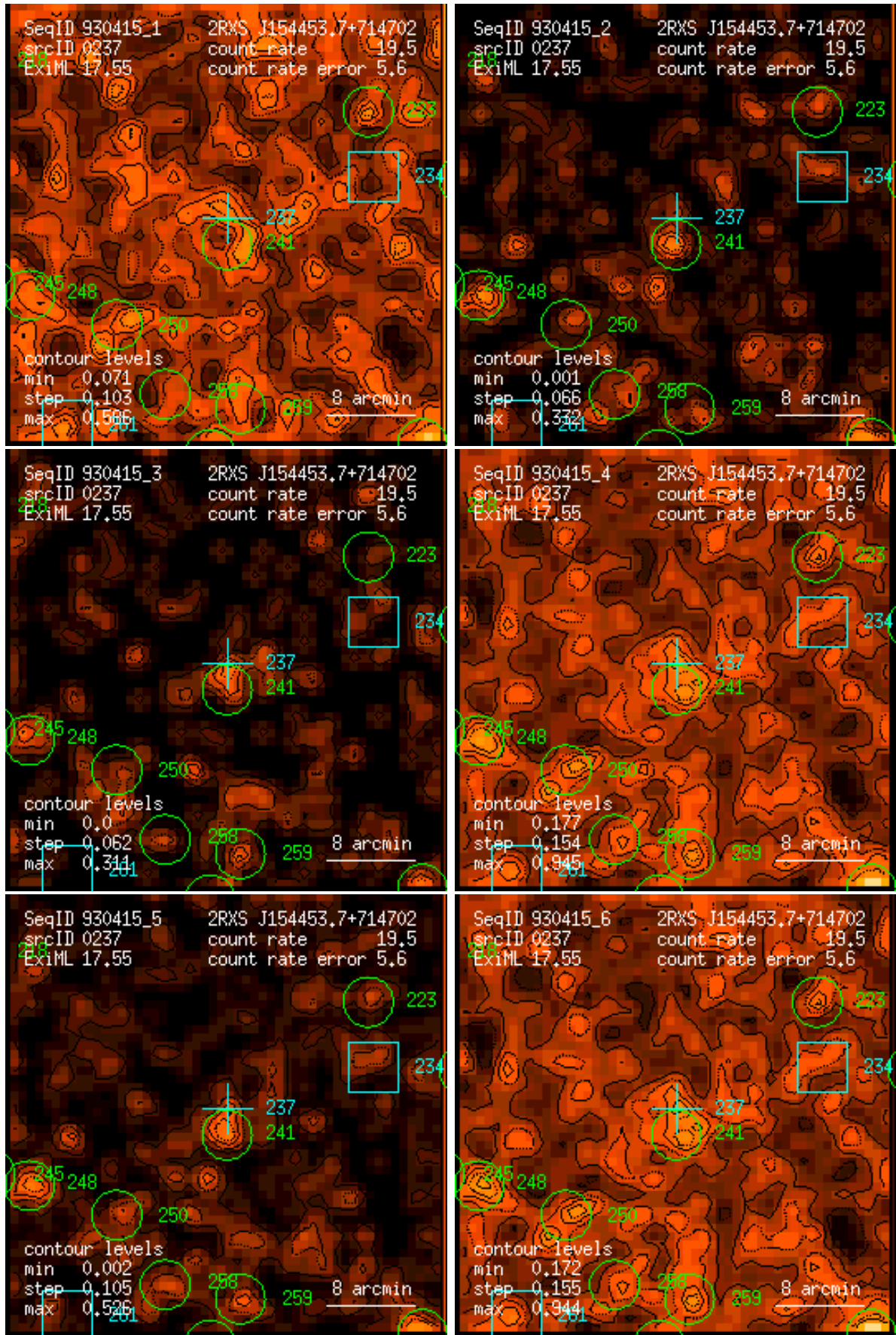
Figure 237: RASS 930415: detection 0237: band rate images, Gaussian filter: (1) PSPC channels 11 – 41, (2) 52 – 90, (3) 91 – 201, (4) 11 – 235, (5) 52 – 201, (6) 11 – 201. Broad band rates in counts/ks. Band rate contour levels in counts/ks/arcmin 2 .
