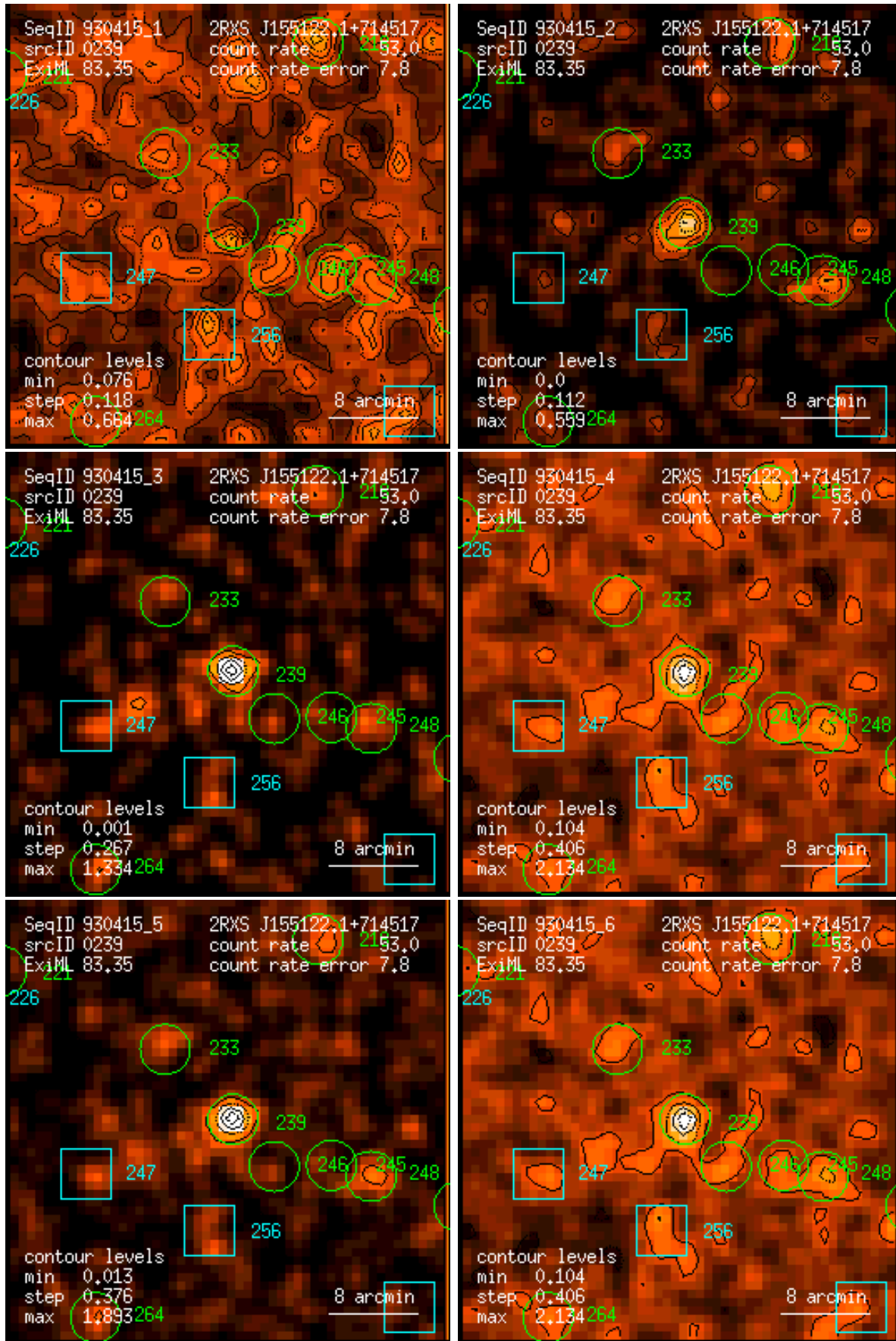
Figure 239: RASS 930415: detection 0239: band rate images, Gaussian filter: (1) PSPC channels 11 – 41, (2) 52 – 90, (3) 91 – 201, (4) 11 – 235, (5) 52 – 201, (6) 11 – 201. Broad band rates in counts/ks. Band rate contour levels in counts/ks/arcmin 2 .
