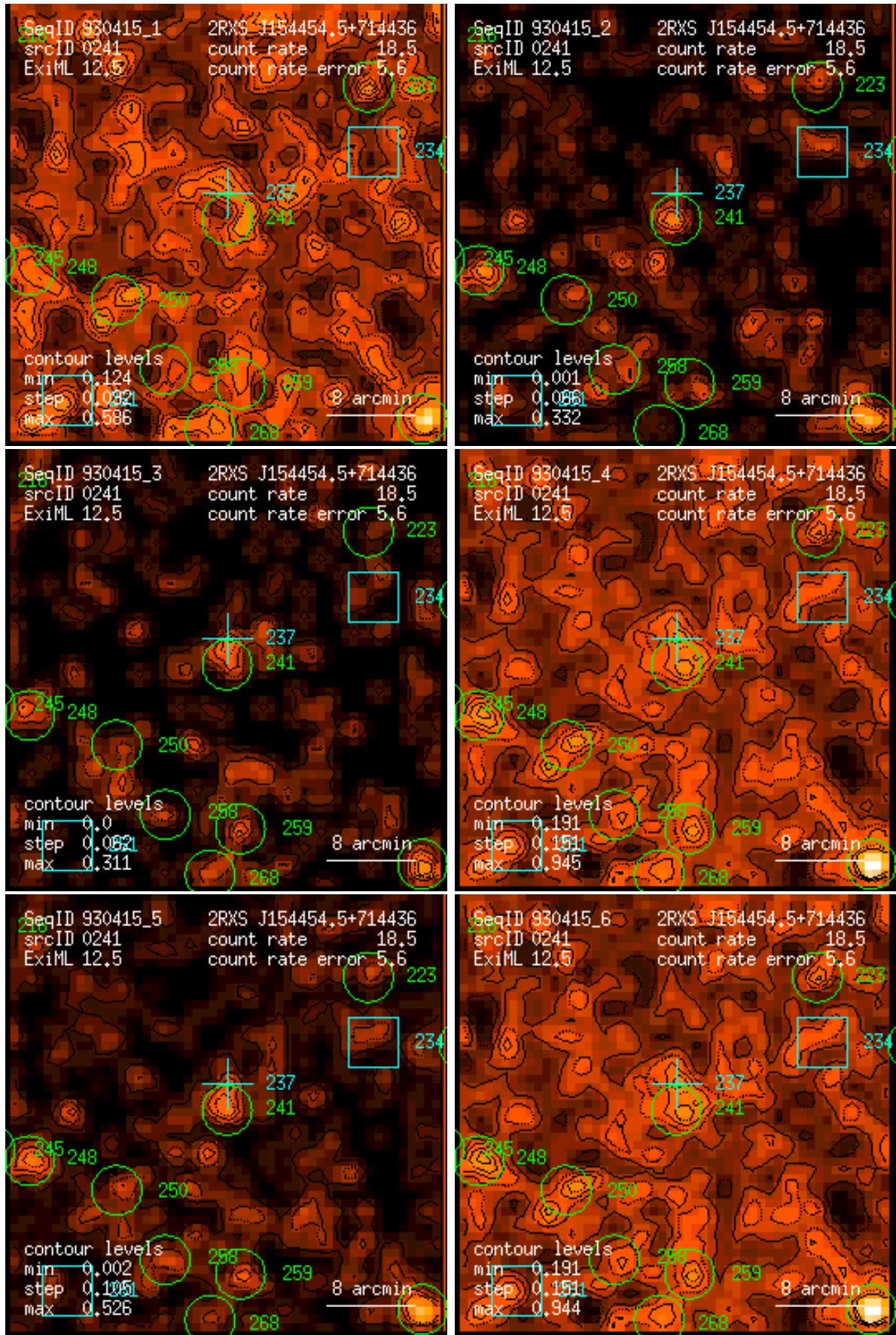
Figure 241: RASS 930415: detection 0241: band rate images, Gaussian filter: (1) PSPC channels 11 – 41, (2) 52 – 90, (3) 91 – 201, (4) 11 – 235, (5) 52 – 201, (6) 11 – 201. Broad band rates in counts/ks. Band rate contour levels in counts/ks/arcmin 2 .
