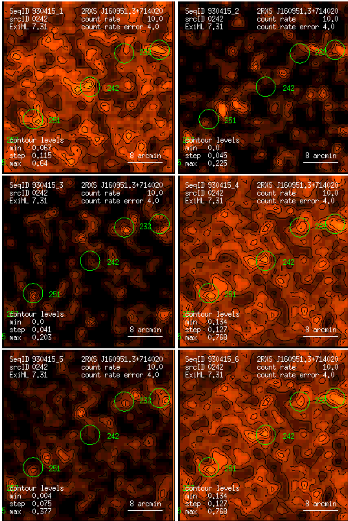
Figure 242: RASS 930415: detection 0242: band rate images, Gaussian filter: (1) PSPC channels 11 – 41, (2) 52 – 90, (3) 91 – 201, (4) 11 – 235, (5) 52 – 201, (6) 11 – 201. Broad band rates in counts/ks. Band rate contour levels in counts/ks/arcmin 2 .
