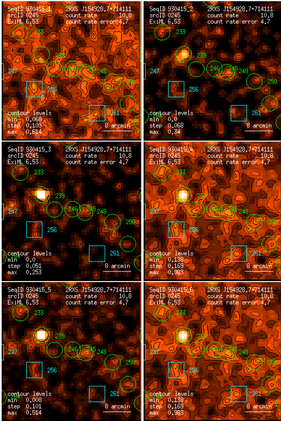
Figure 245: RASS 930415: detection 0245: band rate images, Gaussian filter: (1) PSPC channels 11 – 41, (2) 52 – 90, (3) 91 – 201, (4) 11 – 235, (5) 52 – 201, (6) 11 – 201. Broad band rates in counts/ks. Band rate contour levels in counts/ks/arcmin 2 .
