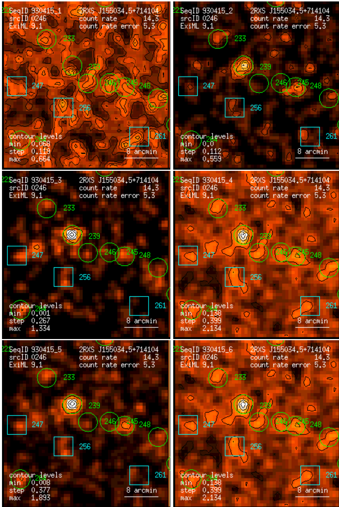
Figure 246: RASS 930415: detection 0246: band rate images, Gaussian filter: (1) PSPC channels 11 – 41, (2) 52 – 90, (3) 91 – 201, (4) 11 – 235, (5) 52 – 201, (6) 11 – 201. Broad band rates in counts/ks. Band rate contour levels in counts/ks/arcmin 2 .
