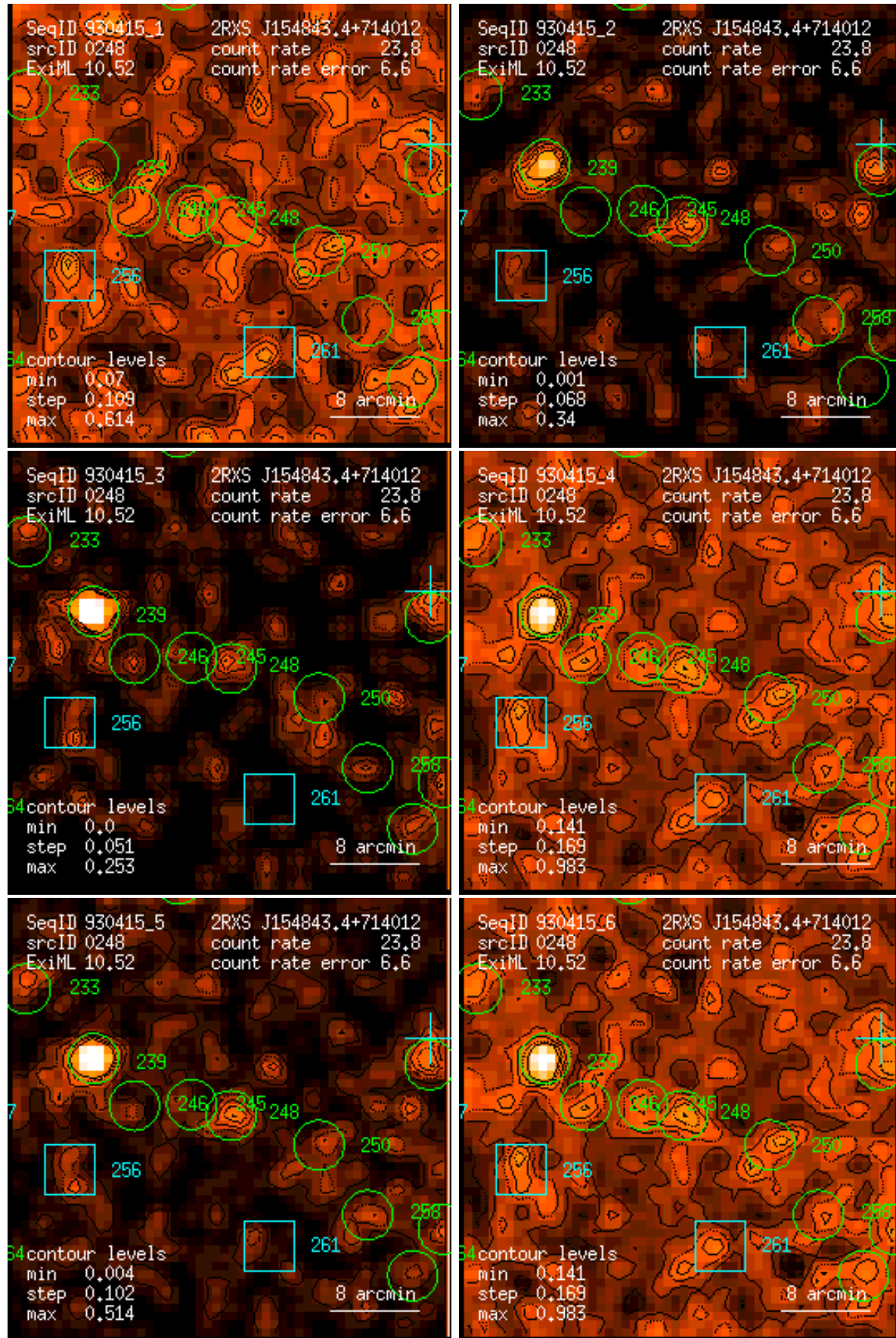
Figure 248: RASS 930415: detection 0248: band rate images, Gaussian filter: (1) PSPC channels 11 – 41, (2) 52 – 90, (3) 91 – 201, (4) 11 – 235, (5) 52 – 201, (6) 11 – 201. Broad band rates in counts/ks. Band rate contour levels in counts/ks/arcmin 2 .
