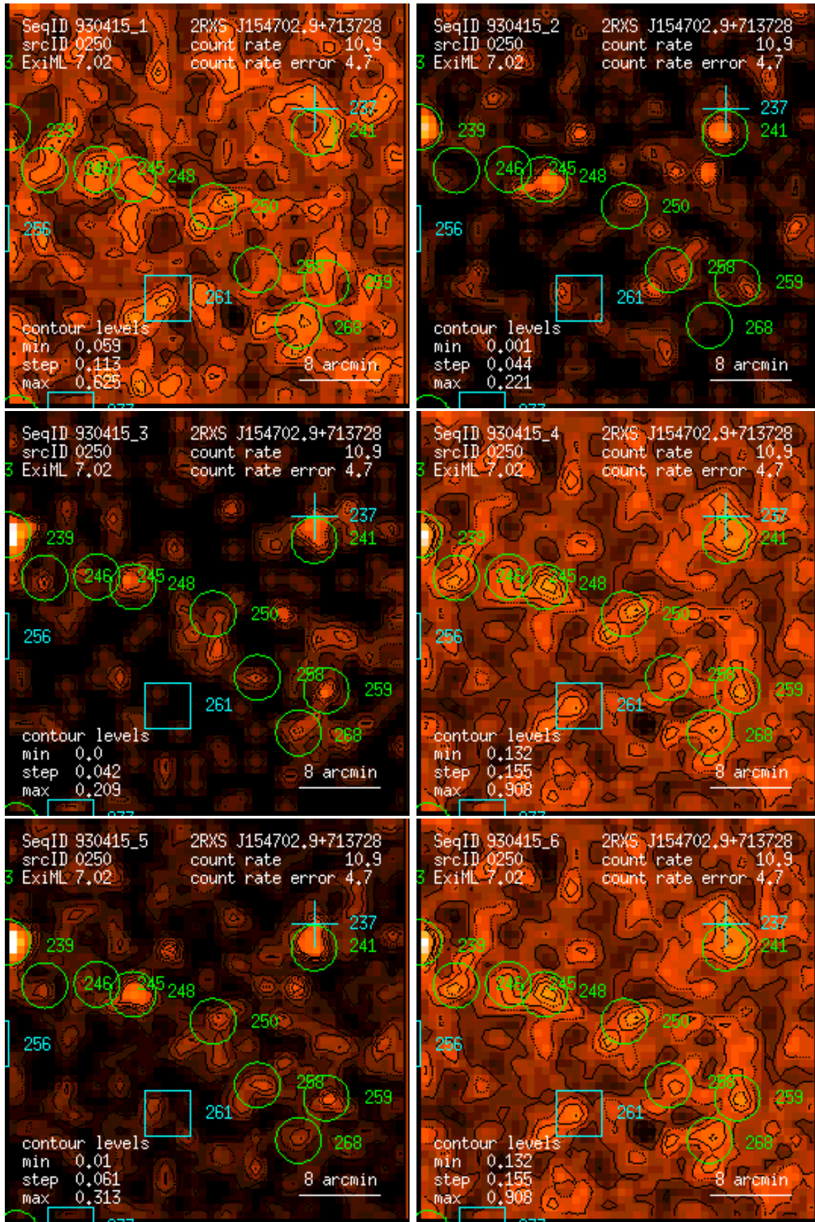
Figure 250: RASS 930415: detection 0250: band rate images, Gaussian filter: (1) PSPC channels 11 – 41, (2) 52 – 90, (3) 91 – 201, (4) 11 – 235, (5) 52 – 201, (6) 11 – 201. Broad band rates in counts/ks. Band rate contour levels in counts/ks/arcmin 2 .
