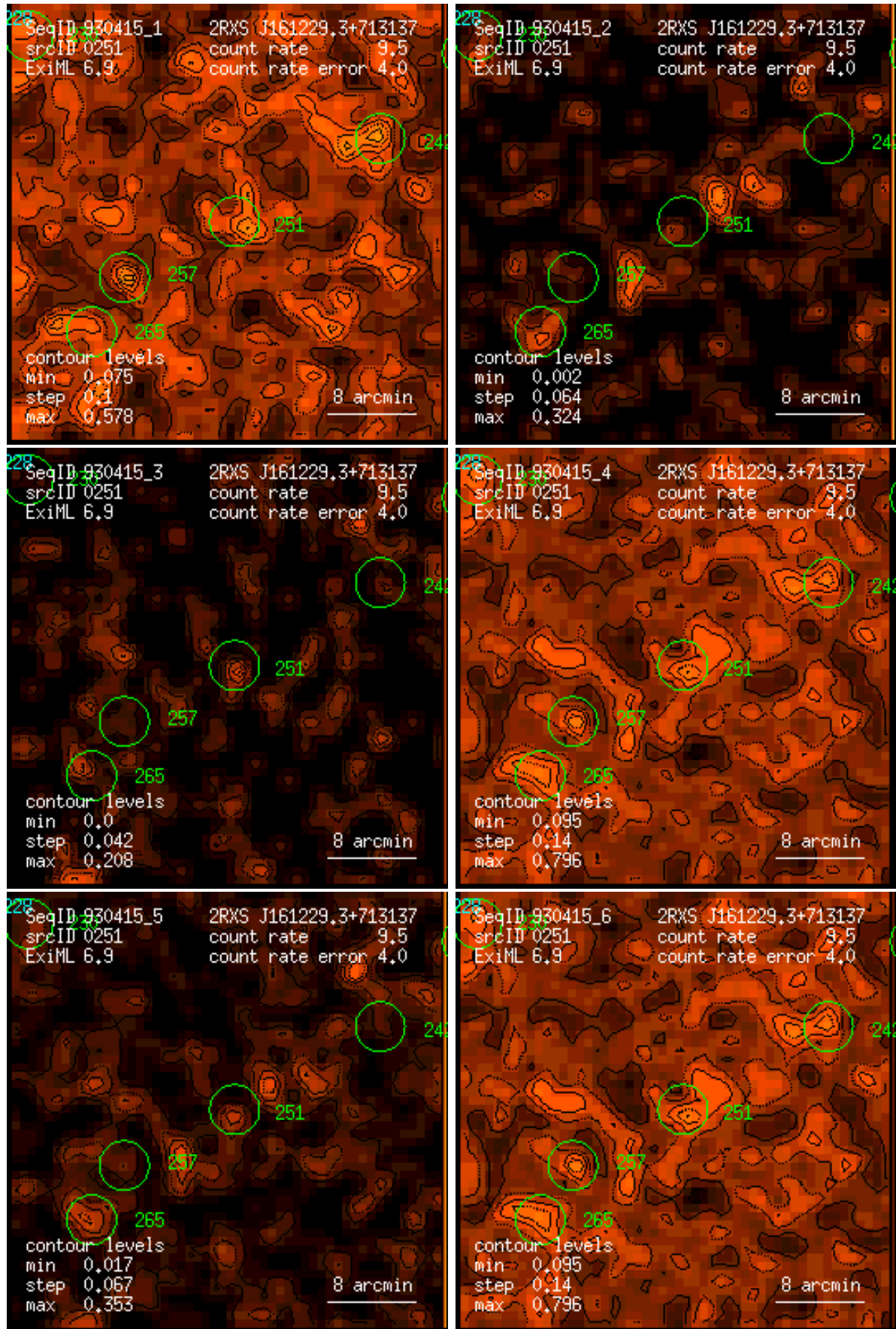
Figure 251: RASS 930415: detection 0251: band rate images, Gaussian filter: (1) PSPC channels 11 – 41, (2) 52 – 90, (3) 91 – 201, (4) 11 – 235, (5) 52 – 201, (6) 11 – 201. Broad band rates in counts/ks. Band rate contour levels in counts/ks/arcmin 2 .
