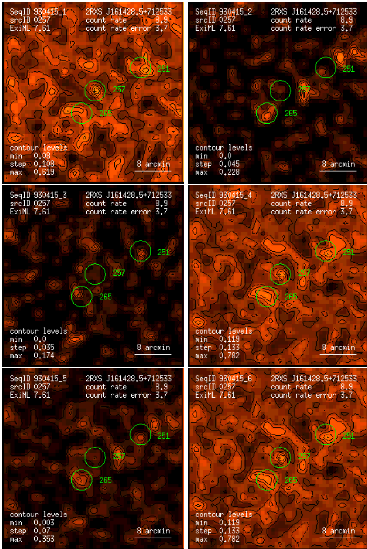
Figure 257: RASS 930415: detection 0257: band rate images, Gaussian filter: (1) PSPC channels 11 – 41, (2) 52 – 90, (3) 91 – 201, (4) 11 – 235, (5) 52 – 201, (6) 11 – 201. Broad band rates in counts/ks. Band rate contour levels in counts/ks/arcmin 2 .
