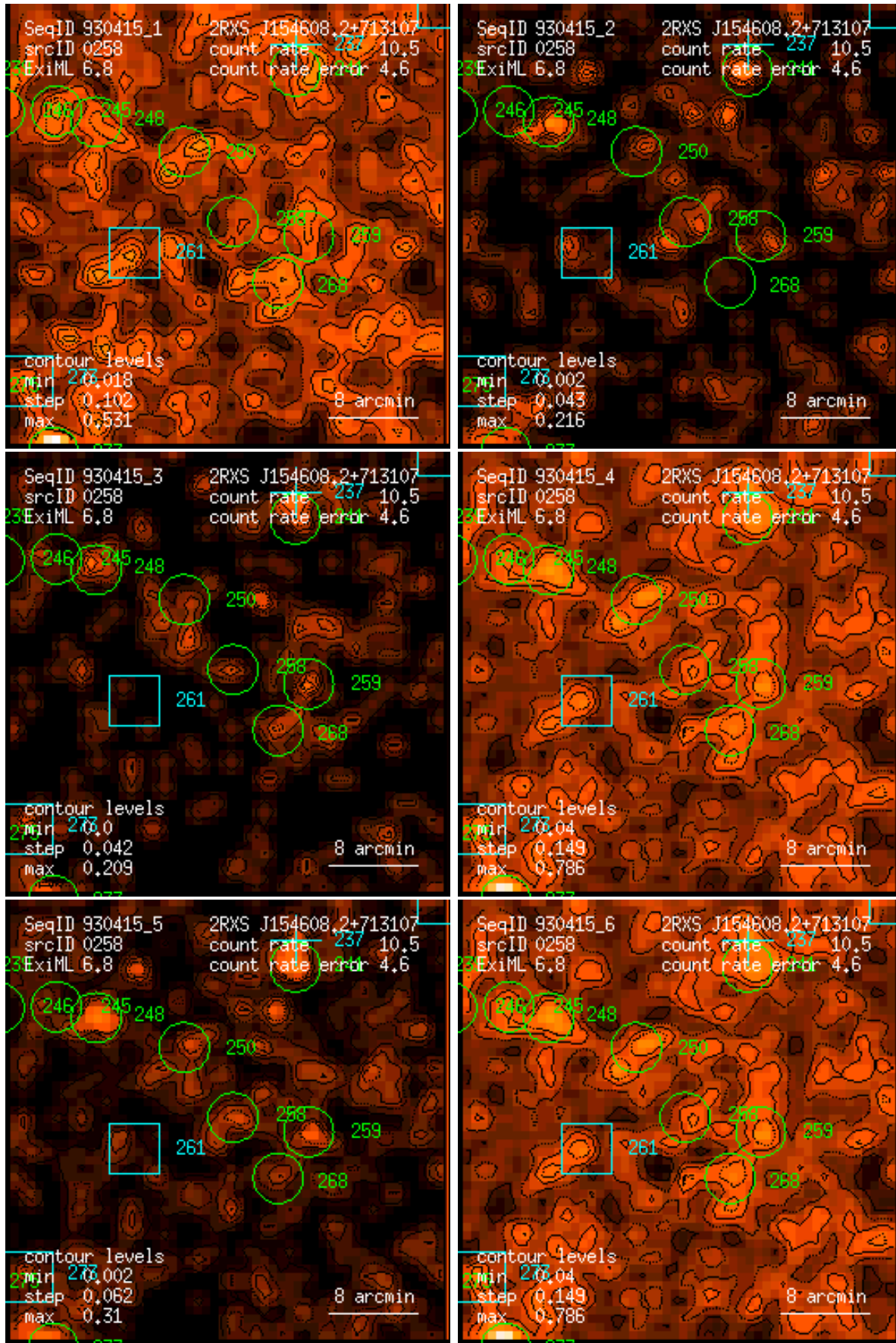
Figure 258: RASS 930415: detection 0258: band rate images, Gaussian filter: (1) PSPC channels 11 – 41, (2) 52 – 90, (3) 91 – 201, (4) 11 – 235, (5) 52 – 201, (6) 11 – 201. Broad band rates in counts/ks. Band rate contour levels in counts/ks/arcmin 2 .
