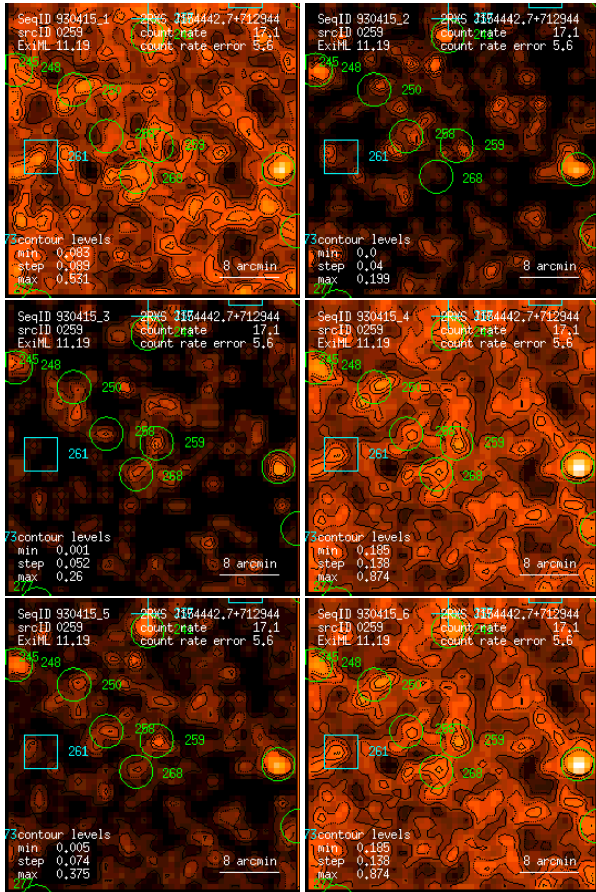
Figure 259: RASS 930415: detection 0259: band rate images, Gaussian filter: (1) PSPC channels 11 – 41, (2) 52 – 90, (3) 91 – 201, (4) 11 – 235, (5) 52 – 201, (6) 11 – 201. Broad band rates in counts/ks. Band rate contour levels in counts/ks/arcmin 2 .
