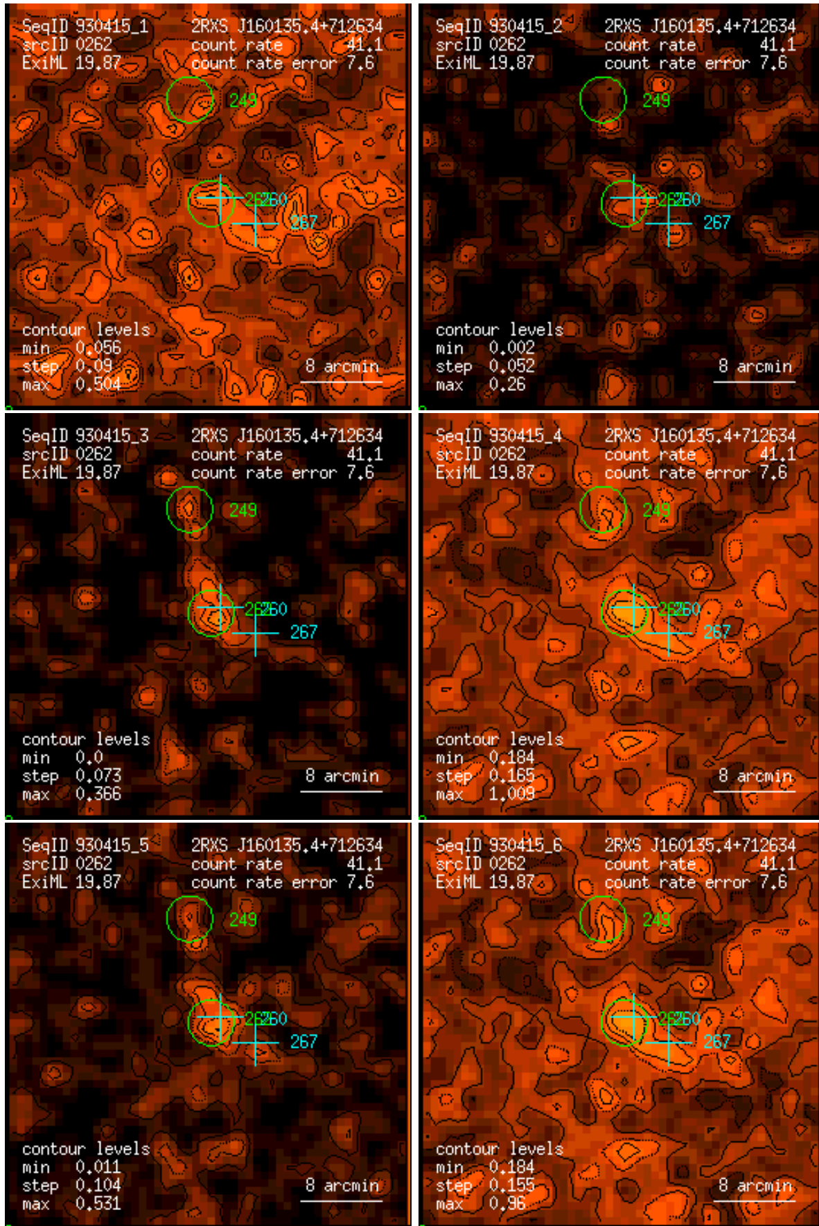
Figure 262: RASS 930415: detection 0262: band rate images, Gaussian filter: (1) PSPC channels 11 – 41, (2) 52 – 90, (3) 91 – 201, (4) 11 – 235, (5) 52 – 201, (6) 11 – 201. Broad band rates in counts/ks. Band rate contour levels in counts/ks/arcmin 2 .
