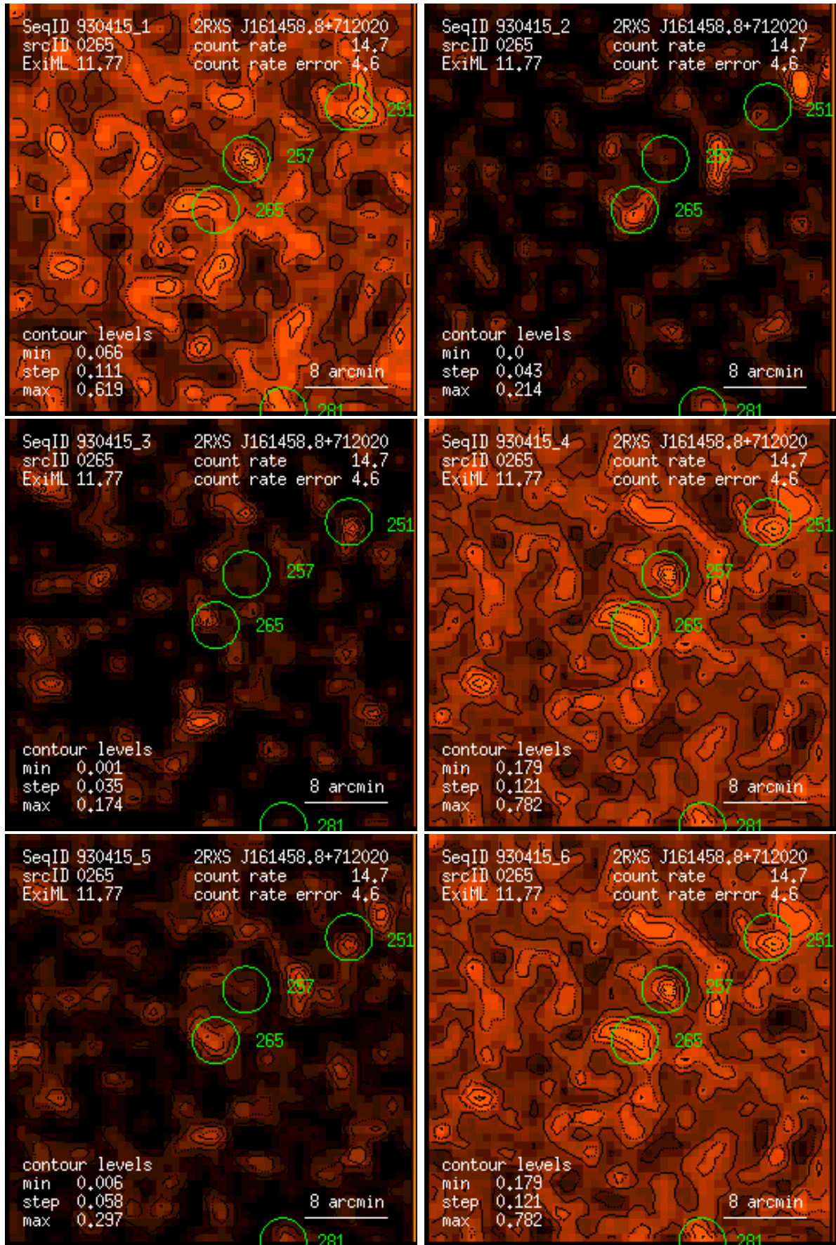
Figure 265: RASS 930415: detection 0265: band rate images, Gaussian filter: (1) PSPC channels 11 – 41, (2) 52 – 90, (3) 91 – 201, (4) 11 – 235, (5) 52 – 201, (6) 11 – 201. Broad band rates in counts/ks. Band rate contour levels in counts/ks/arcmin 2 .
