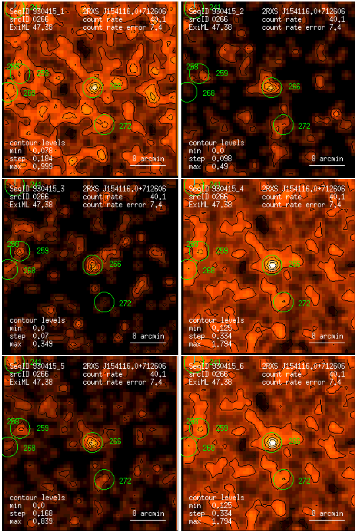
Figure 266: RASS 930415: detection 0266: band rate images, Gaussian filter: (1) PSPC channels 11 – 41, (2) 52 – 90, (3) 91 – 201, (4) 11 – 235, (5) 52 – 201, (6) 11 – 201. Broad band rates in counts/ks. Band rate contour levels in counts/ks/arcmin 2 .
