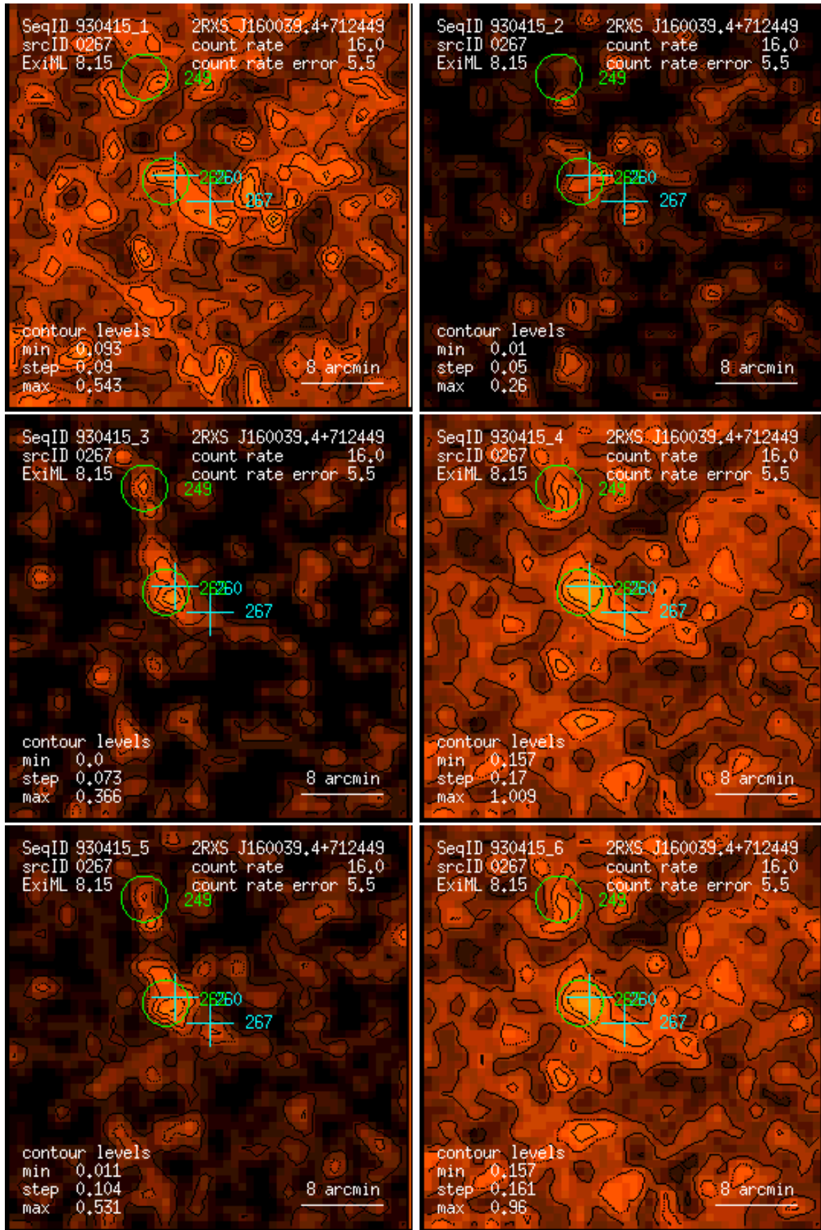
Figure 267: RASS 930415: detection 0267: band rate images, Gaussian filter: (1) PSPC channels 11 – 41, (2) 52 – 90, (3) 91 – 201, (4) 11 – 235, (5) 52 – 201, (6) 11 – 201. Broad band rates in counts/ks. Band rate contour levels in counts/ks/arcmin 2 .
