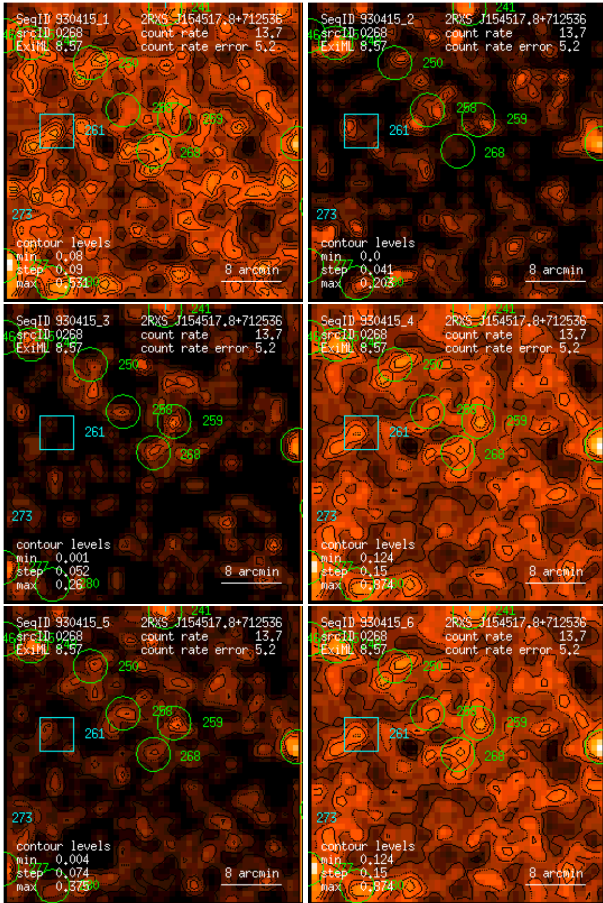
Figure 268: RASS 930415: detection 0268: band rate images, Gaussian filter: (1) PSPC channels 11 – 41, (2) 52 – 90, (3) 91 – 201, (4) 11 – 235, (5) 52 – 201, (6) 11 – 201. Broad band rates in counts/ks. Band rate contour levels in counts/ks/arcmin 2 .
