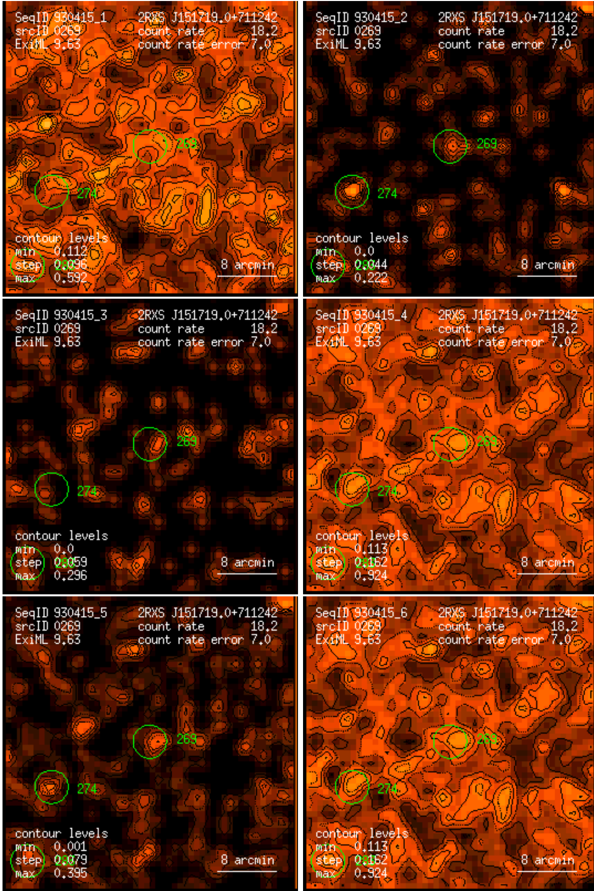
Figure 269: RASS 930415: detection 0269: band rate images, Gaussian filter: (1) PSPC channels 11 – 41, (2) 52 – 90, (3) 91 – 201, (4) 11 – 235, (5) 52 – 201, (6) 11 – 201. Broad band rates in counts/ks. Band rate contour levels in counts/ks/arcmin 2 .
