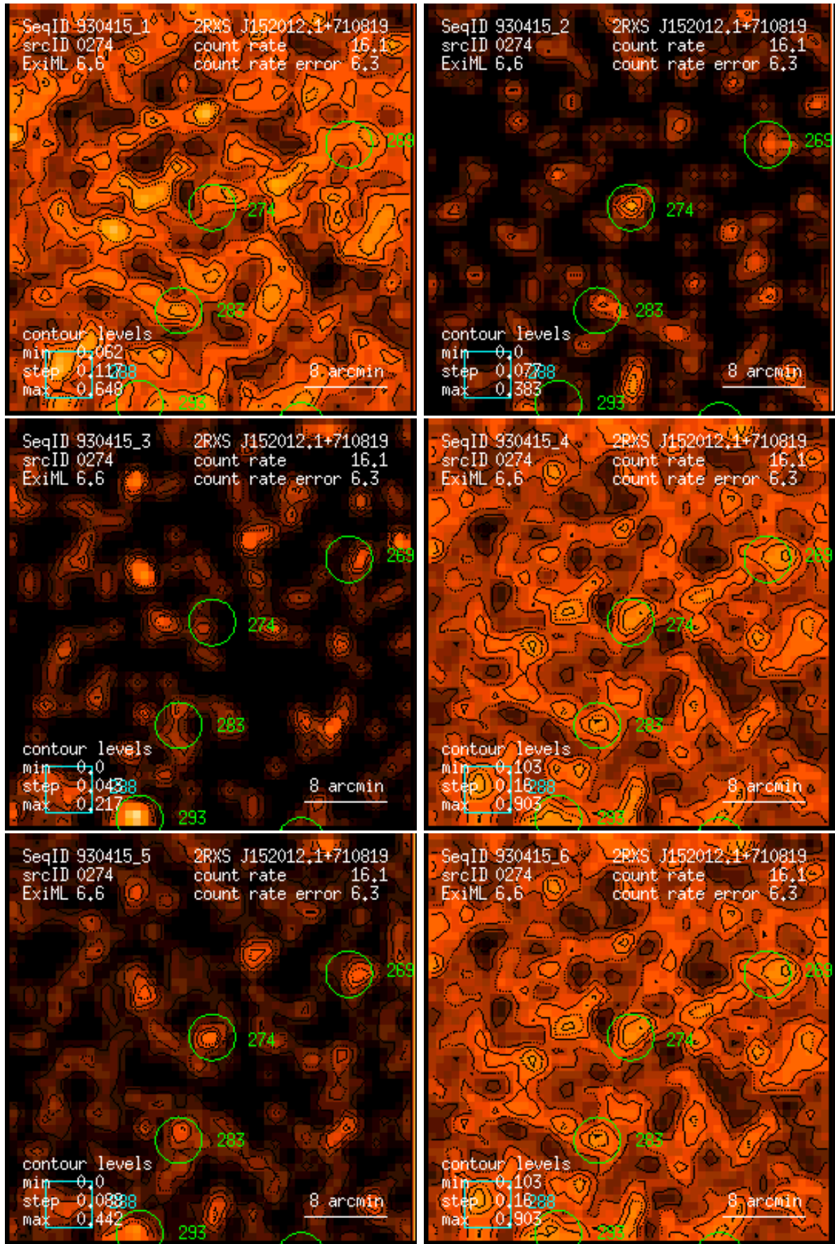
Figure 274: RASS 930415: detection 0274: band rate images, Gaussian filter: (1) PSPC channels 11 – 41, (2) 52 – 90, (3) 91 – 201, (4) 11 – 235, (5) 52 – 201, (6) 11 – 201. Broad band rates in counts/ks. Band rate contour levels in counts/ks/arcmin 2 .
