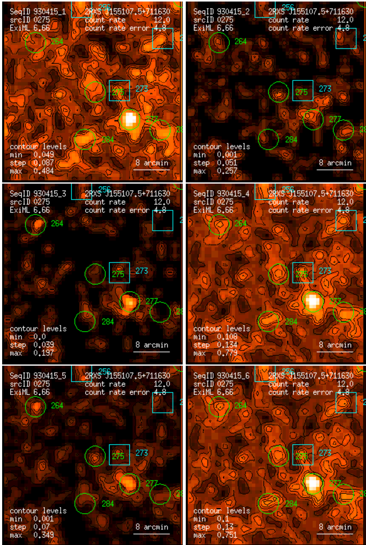
Figure 275: RASS 930415: detection 0275: band rate images, Gaussian filter: (1) PSPC channels 11 – 41, (2) 52 – 90, (3) 91 – 201, (4) 11 – 235, (5) 52 – 201, (6) 11 – 201. Broad band rates in counts/ks. Band rate contour levels in counts/ks/arcmin 2 .
