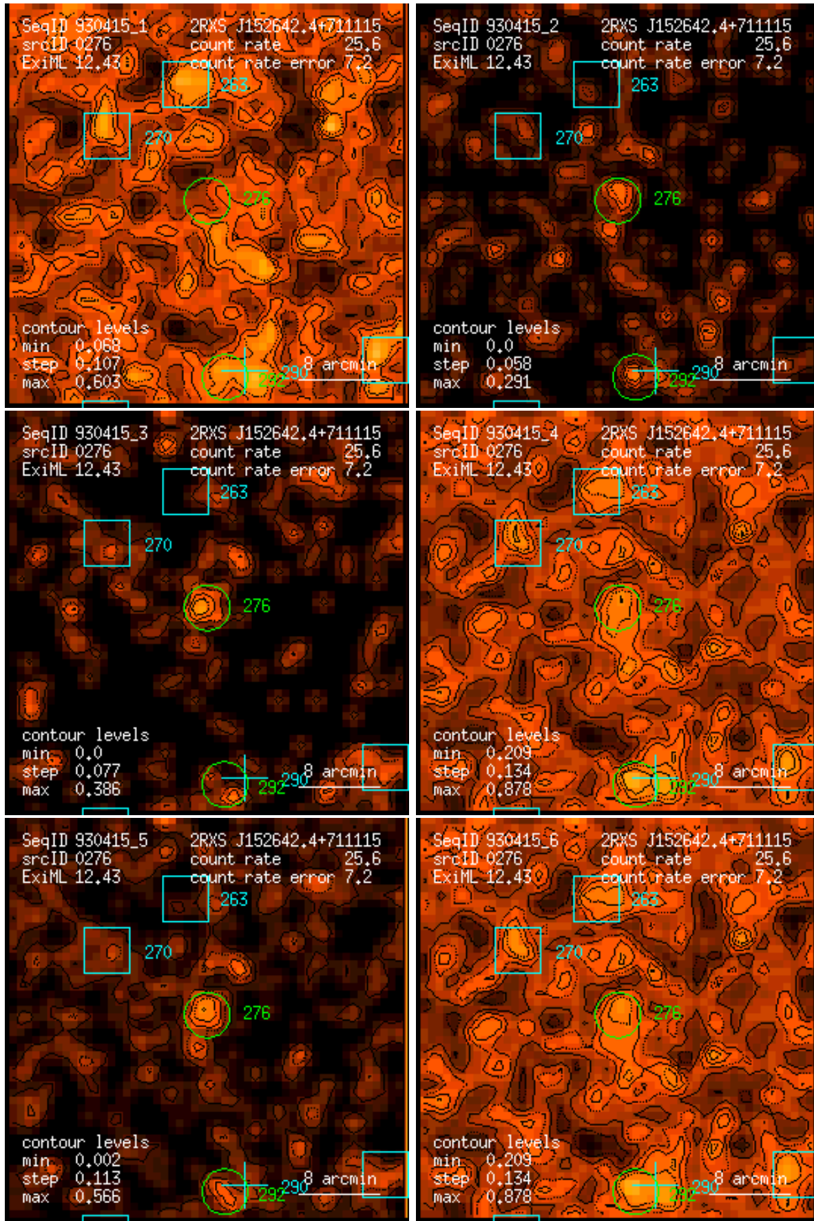
Figure 276: RASS 930415: detection 0276: band rate images, Gaussian filter: (1) PSPC channels 11 – 41, (2) 52 – 90, (3) 91 – 201, (4) 11 – 235, (5) 52 – 201, (6) 11 – 201. Broad band rates in counts/ks. Band rate contour levels in counts/ks/arcmin 2 .
