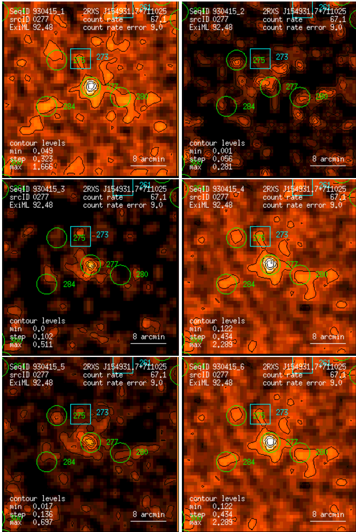
Figure 277: RASS 930415: detection 0277: band rate images, Gaussian filter: (1) PSPC channels 11 – 41, (2) 52 – 90, (3) 91 – 201, (4) 11 – 235, (5) 52 – 201, (6) 11 – 201. Broad band rates in counts/ks. Band rate contour levels in counts/ks/arcmin 2 .
