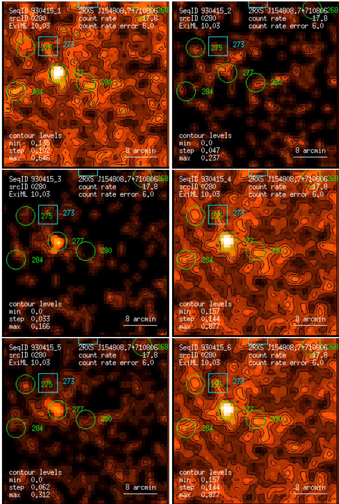
Figure 280: RASS 930415: detection 0280: band rate images, Gaussian filter: (1) PSPC channels 11 – 41, (2) 52 – 90, (3) 91 – 201, (4) 11 – 235, (5) 52 – 201, (6) 11 – 201. Broad band rates in counts/ks. Band rate contour levels in counts/ks/arcmin 2 .
