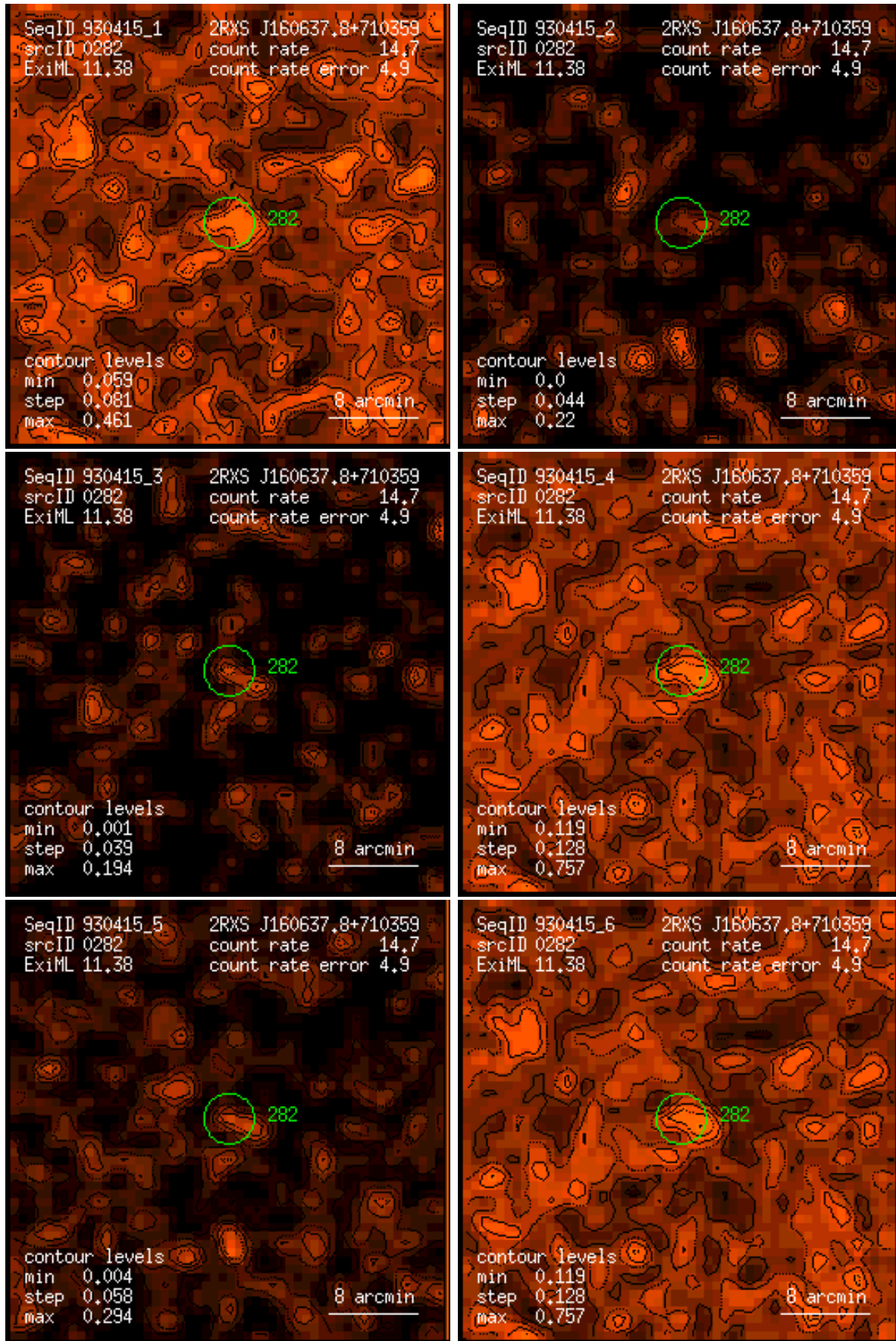
Figure 282: RASS 930415: detection 0282: band rate images, Gaussian filter: (1) PSPC channels 11 – 41, (2) 52 – 90, (3) 91 – 201, (4) 11 – 235, (5) 52 – 201, (6) 11 – 201. Broad band rates in counts/ks. Band rate contour levels in counts/ks/arcmin 2 .
