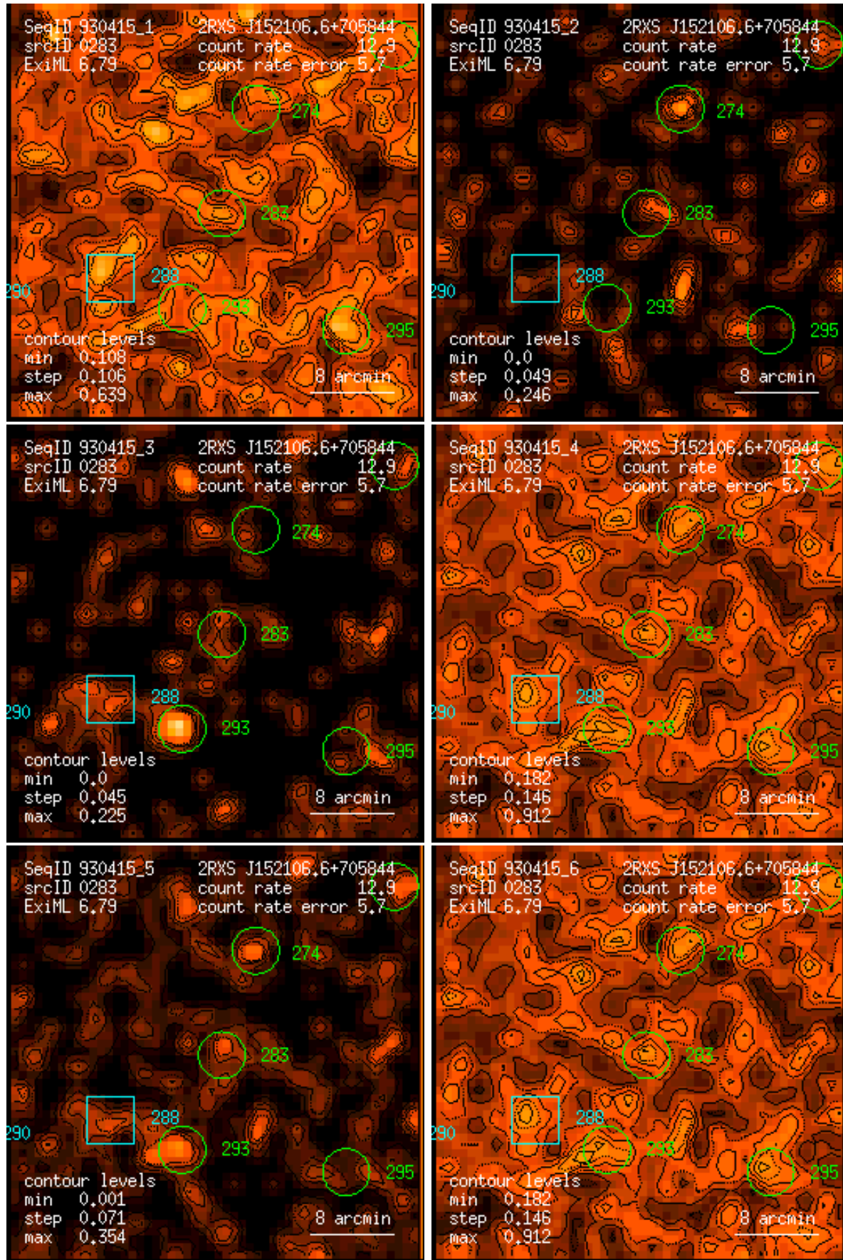
Figure 283: RASS 930415: detection 0283: band rate images, Gaussian filter: (1) PSPC channels 11 – 41, (2) 52 – 90, (3) 91 – 201, (4) 11 – 235, (5) 52 – 201, (6) 11 – 201. Broad band rates in counts/ks. Band rate contour levels in counts/ks/arcmin 2 .
