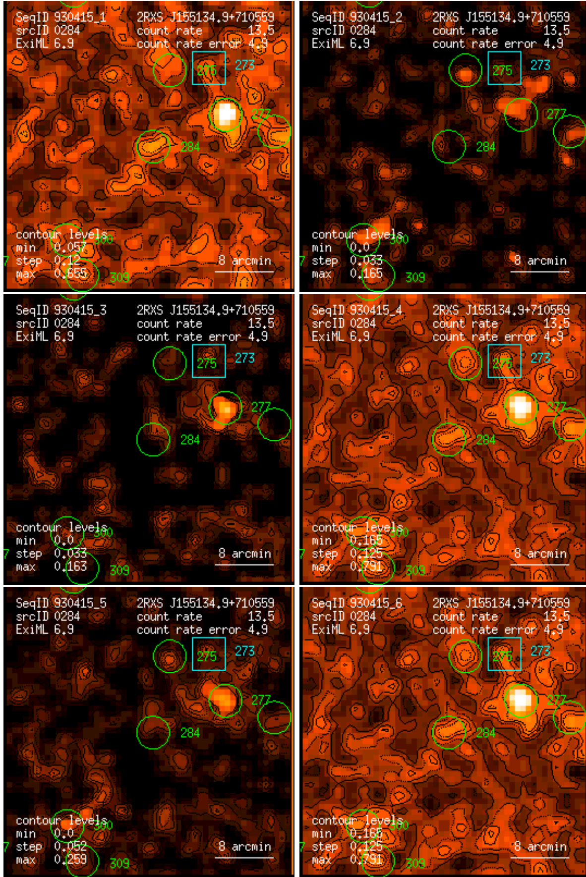
Figure 284: RASS 930415: detection 0284: band rate images, Gaussian filter: (1) PSPC channels 11 – 41, (2) 52 – 90, (3) 91 – 201, (4) 11 – 235, (5) 52 – 201, (6) 11 – 201. Broad band rates in counts/ks. Band rate contour levels in counts/ks/arcmin 2 .
