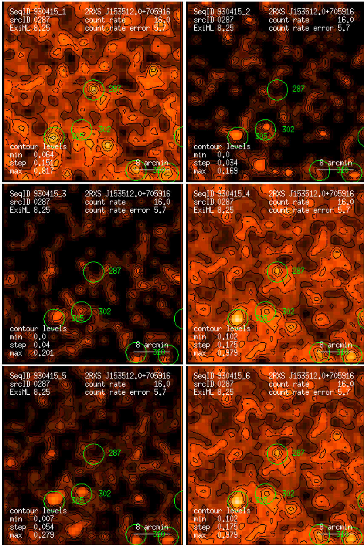
Figure 287: RASS 930415: detection 0287: band rate images, Gaussian filter: (1) PSPC channels 11 – 41, (2) 52 – 90, (3) 91 – 201, (4) 11 – 235, (5) 52 – 201, (6) 11 – 201. Broad band rates in counts/ks. Band rate contour levels in counts/ks/arcmin 2 .
