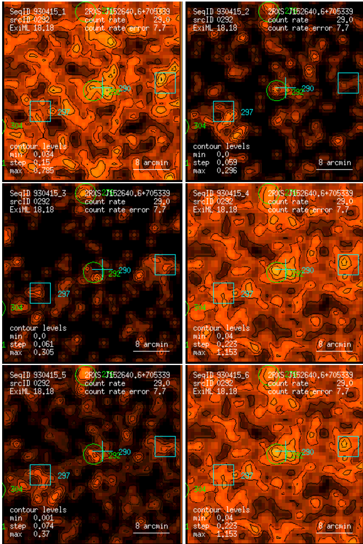
Figure 292: RASS 930415: detection 0292: band rate images, Gaussian filter: (1) PSPC channels 11 – 41, (2) 52 – 90, (3) 91 – 201, (4) 11 – 235, (5) 52 – 201, (6) 11 – 201. Broad band rates in counts/ks. Band rate contour levels in counts/ks/arcmin 2 .
