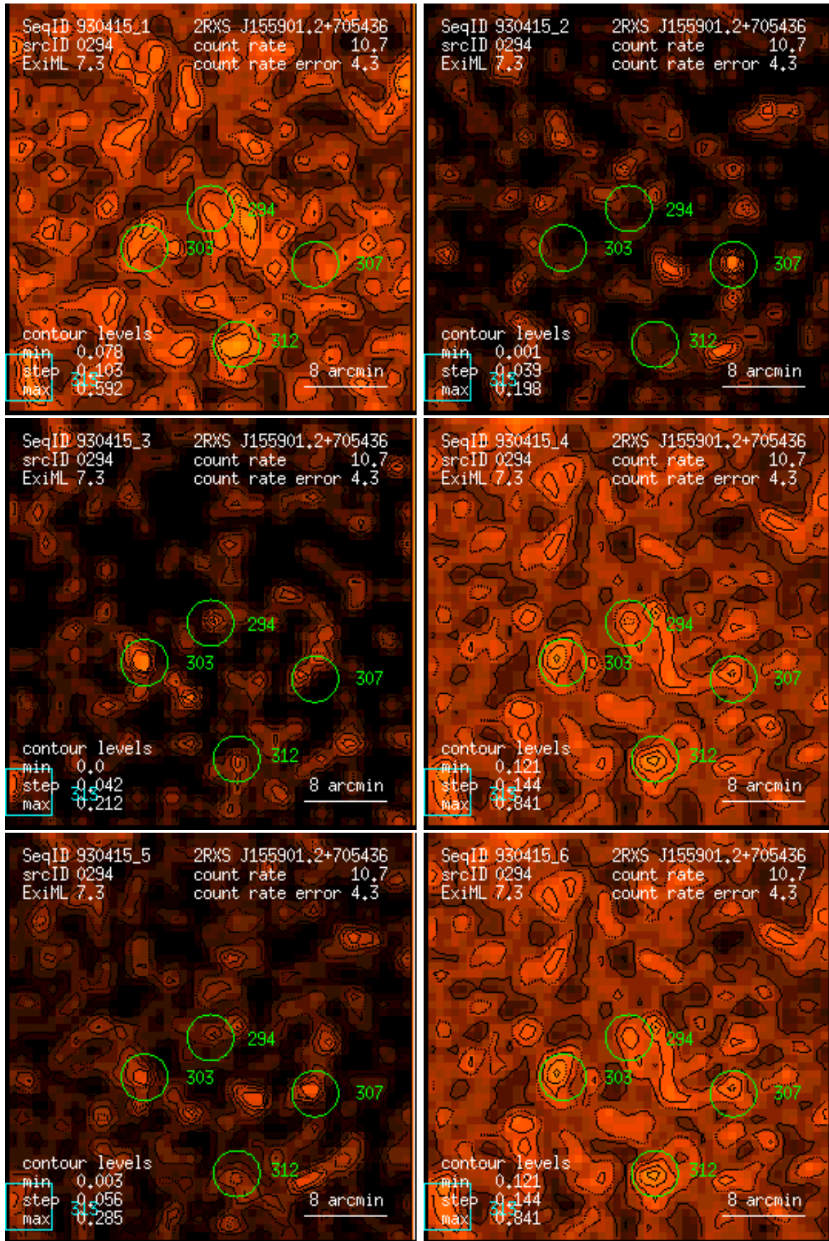
Figure 294: RASS 930415: detection 0294: band rate images, Gaussian filter: (1) PSPC channels 11 – 41, (2) 52 – 90, (3) 91 – 201, (4) 11 – 235, (5) 52 – 201, (6) 11 – 201. Broad band rates in counts/ks. Band rate contour levels in counts/ks/arcmin 2 .
