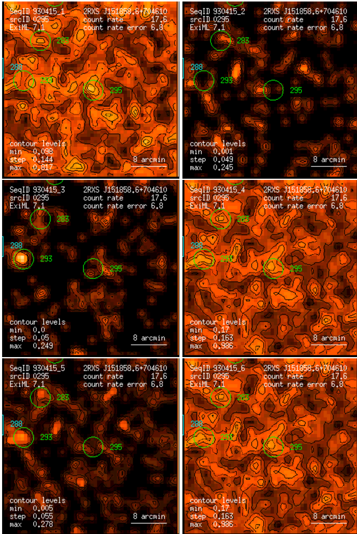
Figure 295: RASS 930415: detection 0295: band rate images, Gaussian filter: (1) PSPC channels 11 – 41, (2) 52 – 90, (3) 91 – 201, (4) 11 – 235, (5) 52 – 201, (6) 11 – 201. Broad band rates in counts/ks. Band rate contour levels in counts/ks/arcmin 2 .
