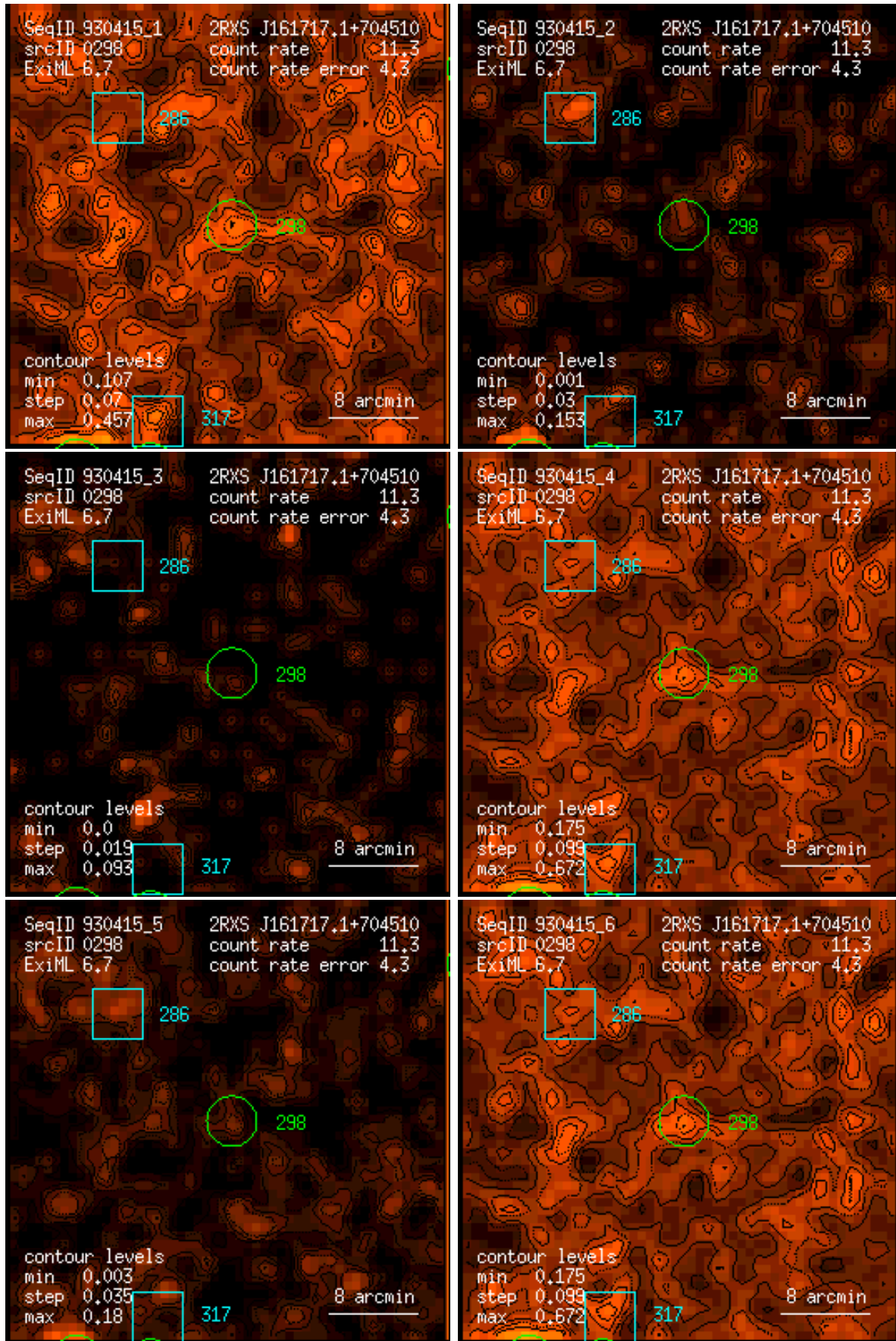
Figure 298: RASS 930415: detection 0298: band rate images, Gaussian filter: (1) PSPC channels 11 – 41, (2) 52 – 90, (3) 91 – 201, (4) 11 – 235, (5) 52 – 201, (6) 11 – 201. Broad band rates in counts/ks. Band rate contour levels in counts/ks/arcmin 2 .
