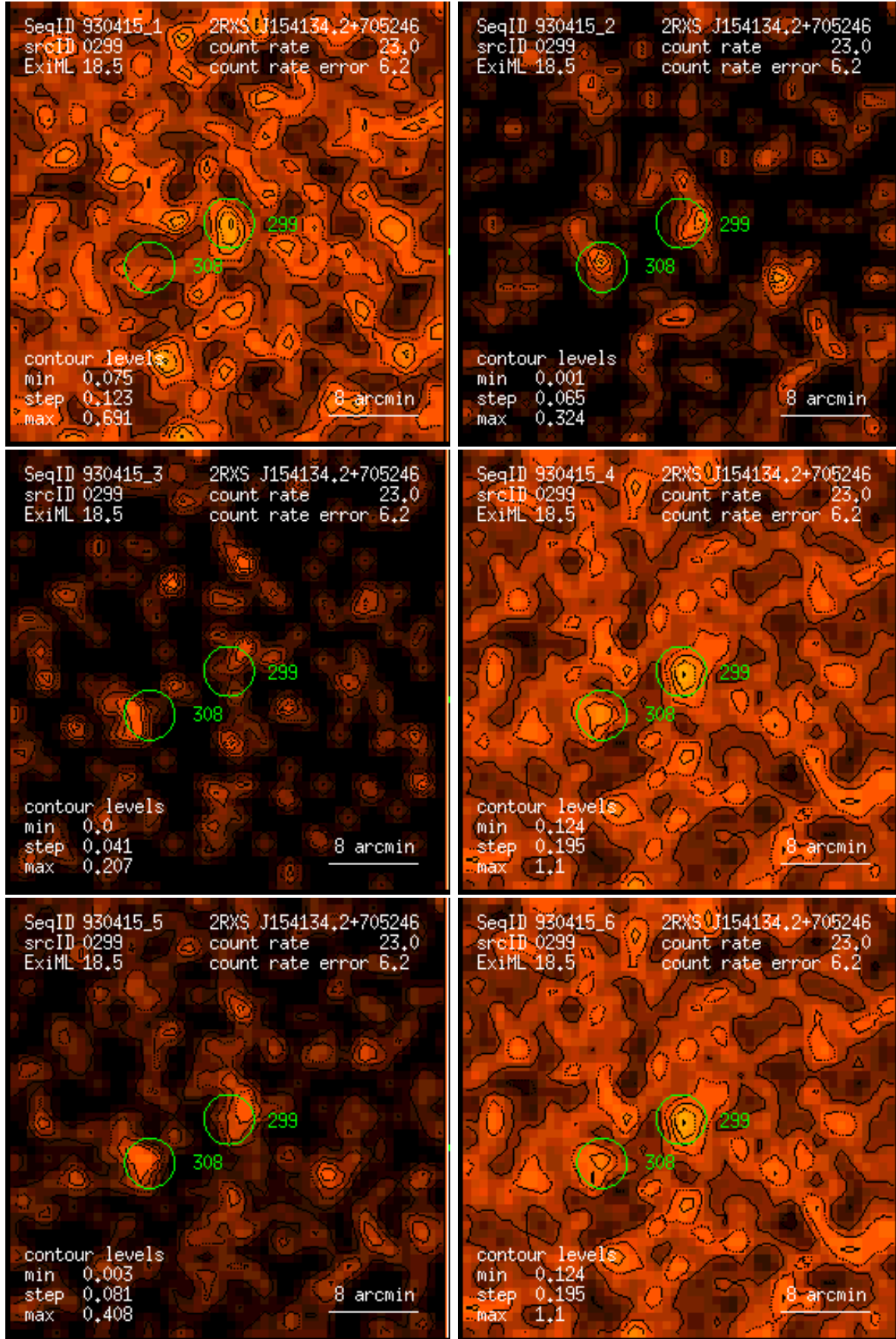
Figure 299: RASS 930415: detection 0299: band rate images, Gaussian filter: (1) PSPC channels 11 – 41, (2) 52 – 90, (3) 91 – 201, (4) 11 – 235, (5) 52 – 201, (6) 11 – 201. Broad band rates in counts/ks. Band rate contour levels in counts/ks/arcmin 2 .
