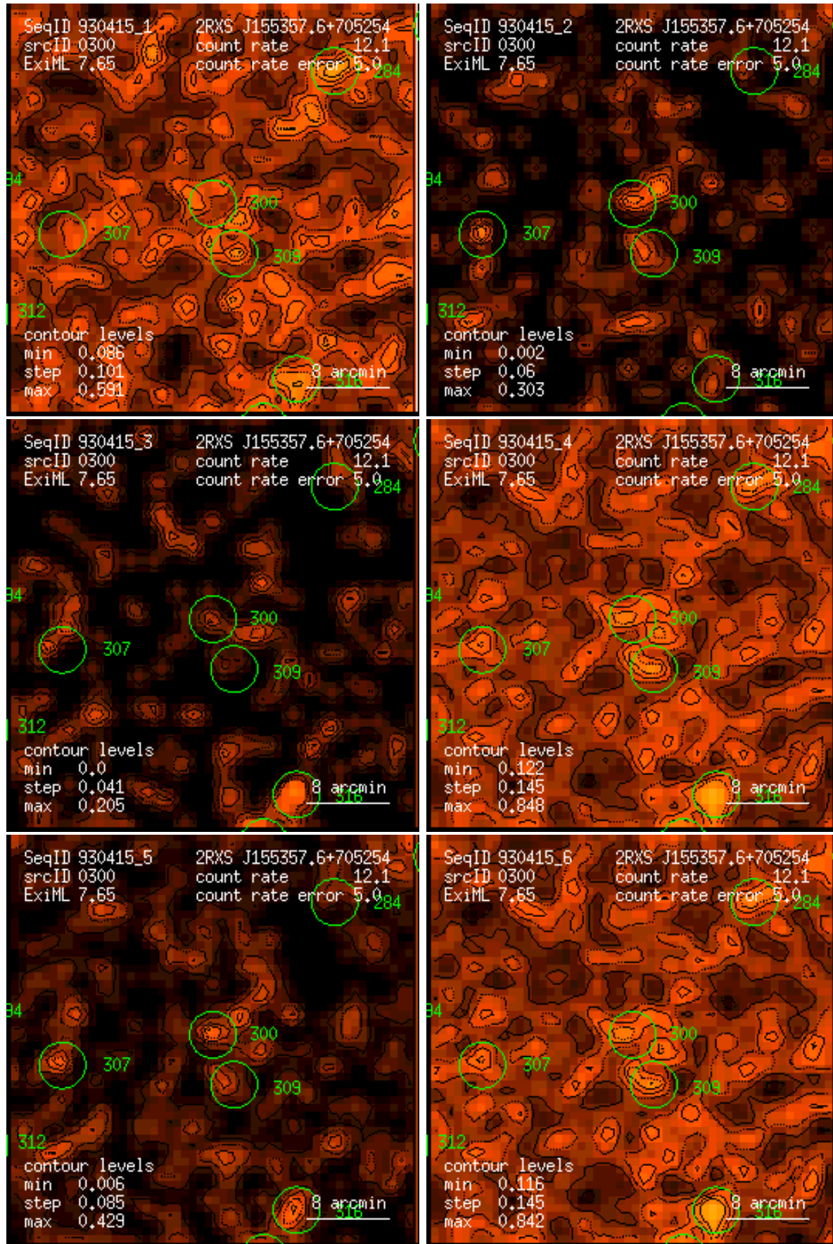
Figure 300: RASS 930415: detection 0300: band rate images, Gaussian filter: (1) PSPC channels 11 – 41, (2) 52 – 90, (3) 91 – 201, (4) 11 – 235, (5) 52 – 201, (6) 11 – 201. Broad band rates in counts/ks. Band rate contour levels in counts/ks/arcmin 2 .
