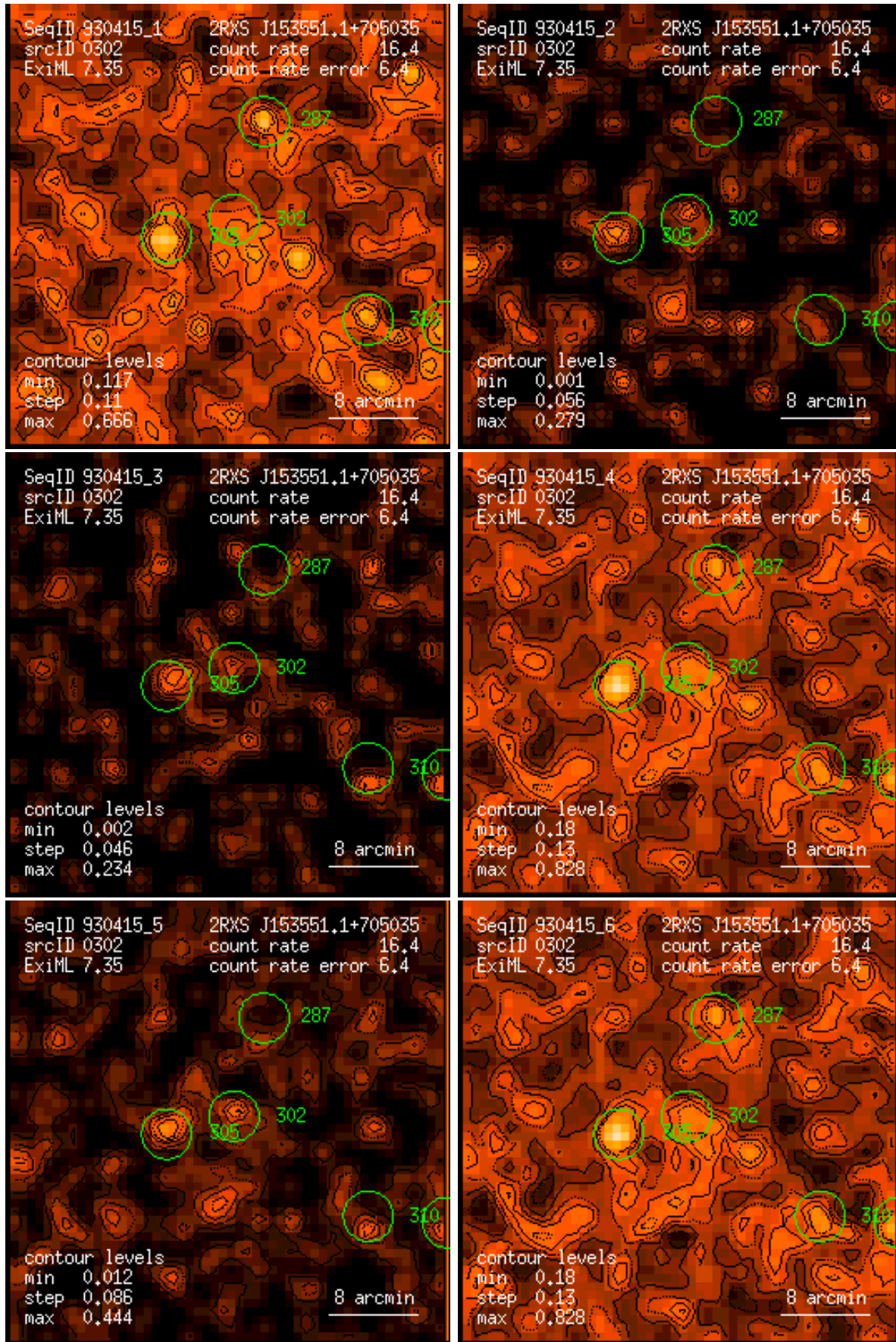
Figure 302: RASS 930415: detection 0302: band rate images, Gaussian filter: (1) PSPC channels 11 – 41, (2) 52 – 90, (3) 91 – 201, (4) 11 – 235, (5) 52 – 201, (6) 11 – 201. Broad band rates in counts/ks. Band rate contour levels in counts/ks/arcmin 2 .
