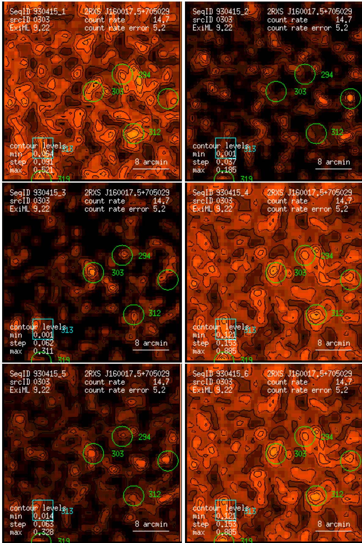
Figure 303: RASS 930415: detection 0303: band rate images, Gaussian filter: (1) PSPC channels 11 – 41, (2) 52 – 90, (3) 91 – 201, (4) 11 – 235, (5) 52 – 201, (6) 11 – 201. Broad band rates in counts/ks. Band rate contour levels in counts/ks/arcmin 2 .
