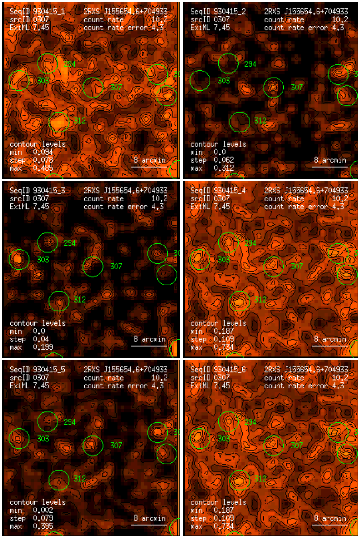
Figure 307: RASS 930415: detection 0307: band rate images, Gaussian filter: (1) PSPC channels 11 – 41, (2) 52 – 90, (3) 91 – 201, (4) 11 – 235, (5) 52 – 201, (6) 11 – 201. Broad band rates in counts/ks. Band rate contour levels in counts/ks/arcmin 2 .
