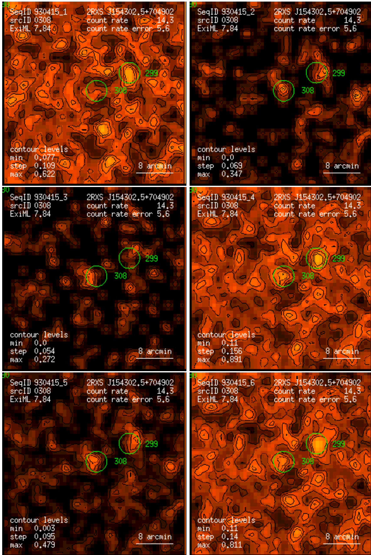
Figure 308: RASS 930415: detection 0308: band rate images, Gaussian filter: (1) PSPC channels 11 – 41, (2) 52 – 90, (3) 91 – 201, (4) 11 – 235, (5) 52 – 201, (6) 11 – 201. Broad band rates in counts/ks. Band rate contour levels in counts/ks/arcmin 2 .
