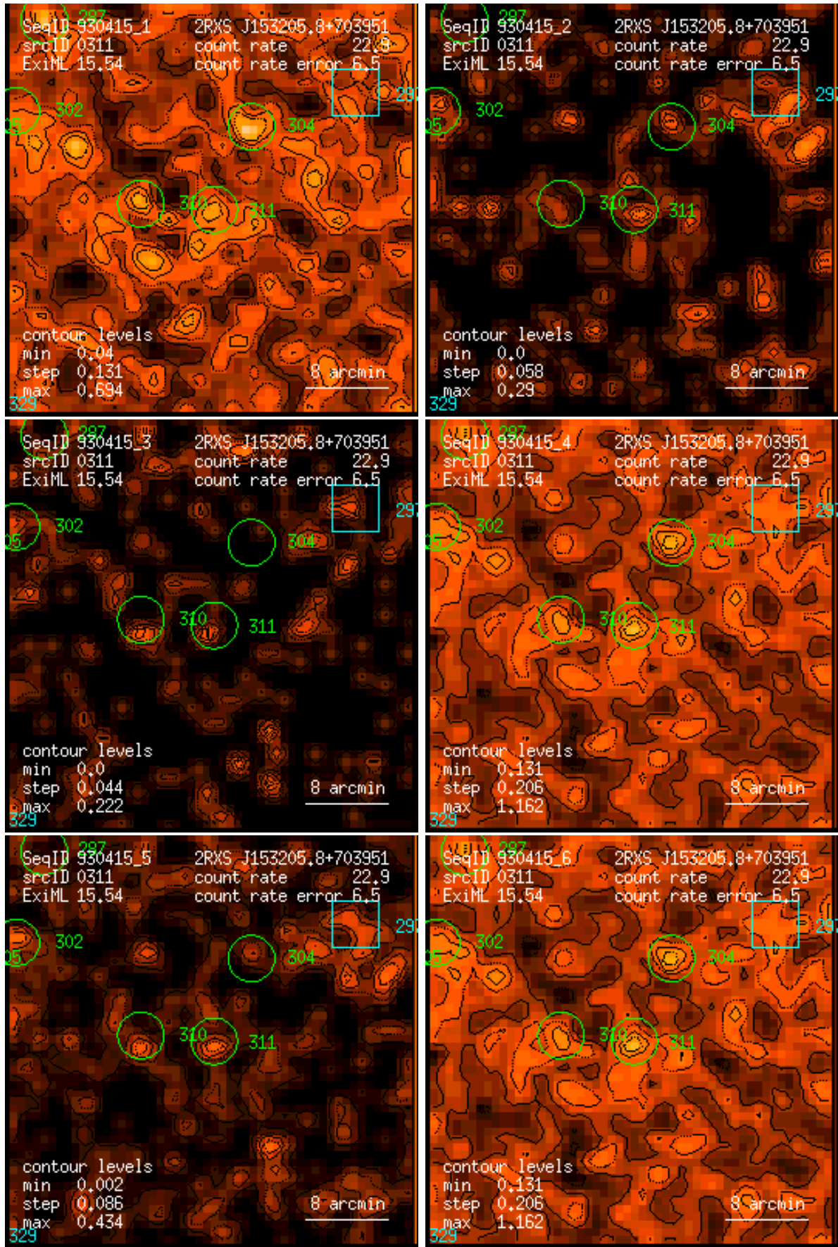
Figure 311: RASS 930415: detection 0311: band rate images, Gaussian filter: (1) PSPC channels 11 – 41, (2) 52 – 90, (3) 91 – 201, (4) 11 – 235, (5) 52 – 201, (6) 11 – 201. Broad band rates in counts/ks. Band rate contour levels in counts/ks/arcmin 2 .
