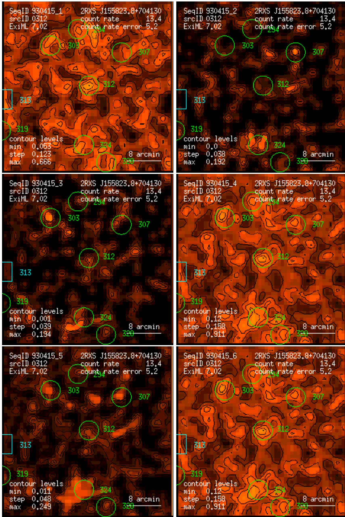
Figure 312: RASS 930415: detection 0312: band rate images, Gaussian filter: (1) PSPC channels 11 – 41, (2) 52 – 90, (3) 91 – 201, (4) 11 – 235, (5) 52 – 201, (6) 11 – 201. Broad band rates in counts/ks. Band rate contour levels in counts/ks/arcmin 2 .
