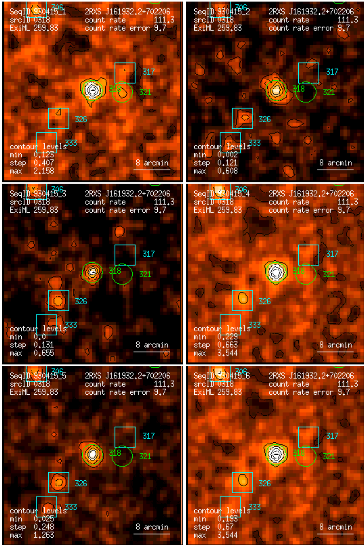
Figure 318: RASS 930415: detection 0318: band rate images, Gaussian filter: (1) PSPC channels 11 – 41, (2) 52 – 90, (3) 91 – 201, (4) 11 – 235, (5) 52 – 201, (6) 11 – 201. Broad band rates in counts/ks. Band rate contour levels in counts/ks/arcmin 2 .
